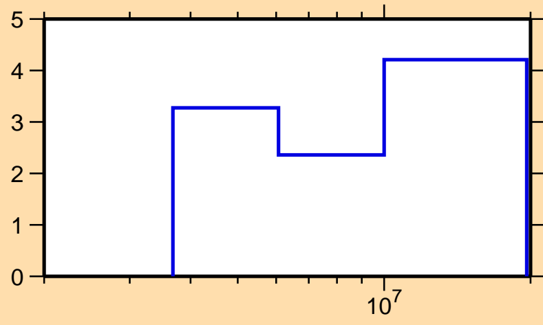
\Delta\sigma/\sigma vs. E for ^{86}\text{Sr}(n,el.)
