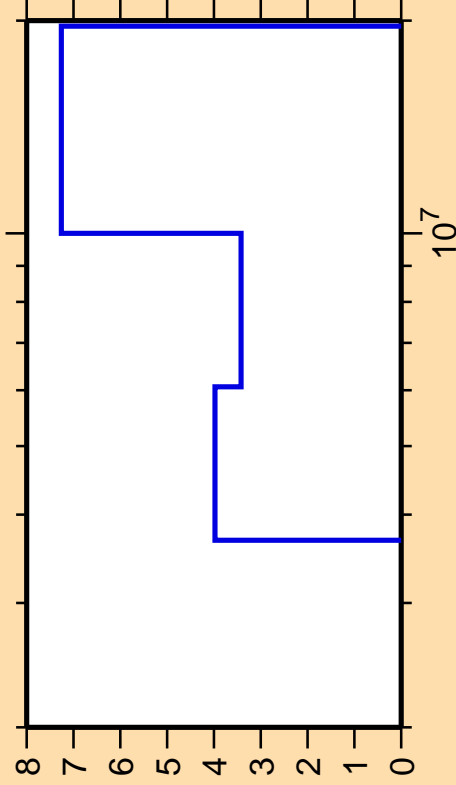
\Delta\sigma/\sigma vs. E for ^{86}\text{Sr}(n,ncont.)
