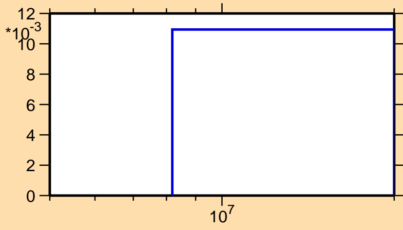
\sigma vs. E for ^{87}\text{Sr}(n,np)
