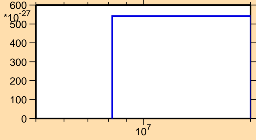
\sigma vs. E for ^{87}\text{Sr}(n,nt)
