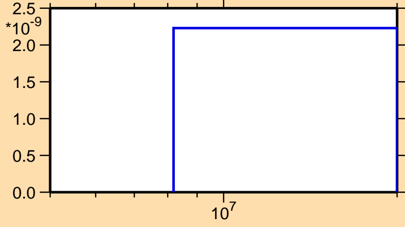
\sigma vs. E for ^{87}\text{Sr}(n,3n)
