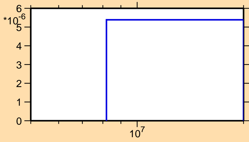
\sigma vs. E for ^{87}\text{Sr}(n,t)
