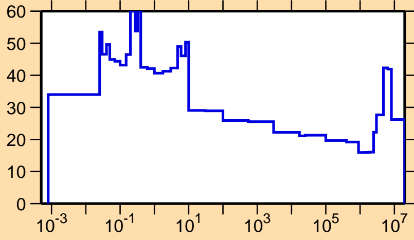
\Delta\sigma/\sigma vs. E for ^{87}\text{Sr}(n,p)
