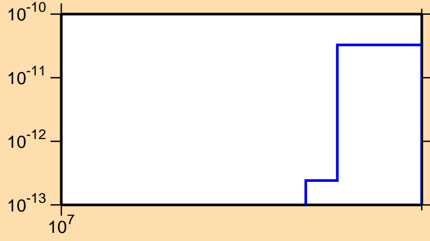
\sigma vs. E for ^{88}\text{Sr}(n,\text{He}3)
