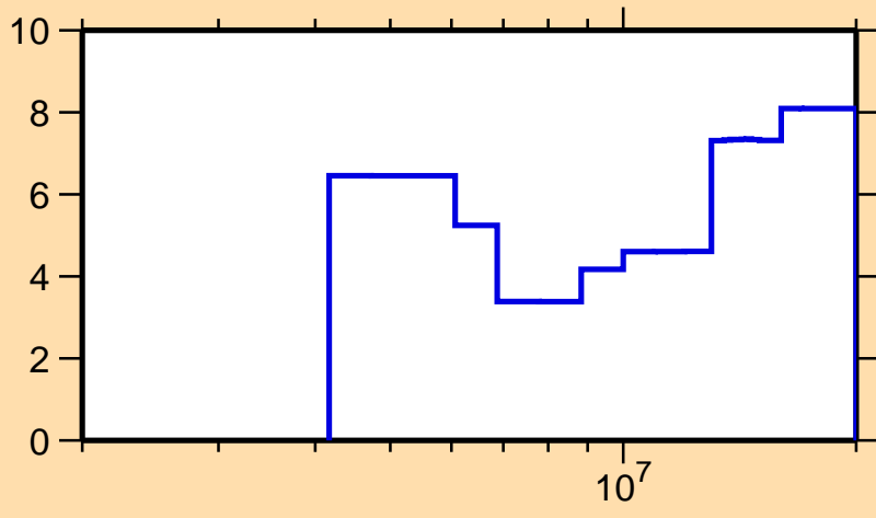
\Delta\sigma/\sigma vs. E for ^{88}\text{Sr}(n,n\text{cont.})
