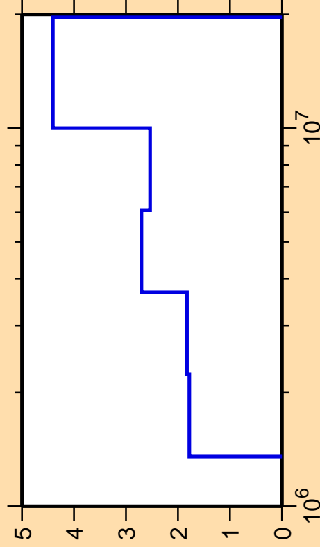
\Delta\sigma/\sigma vs. E for ^{88}\text{Sr}(n,\text{inel.})
