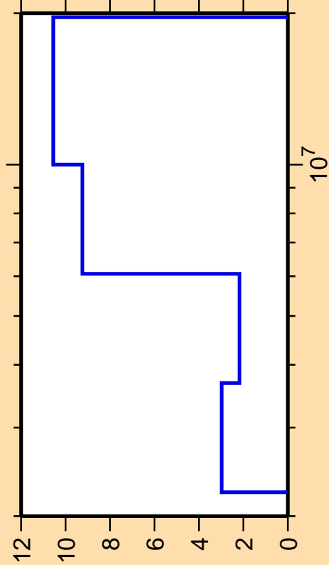
\Delta\sigma/\sigma vs. E for ^{88}\text{Sr}(n,n_2)
