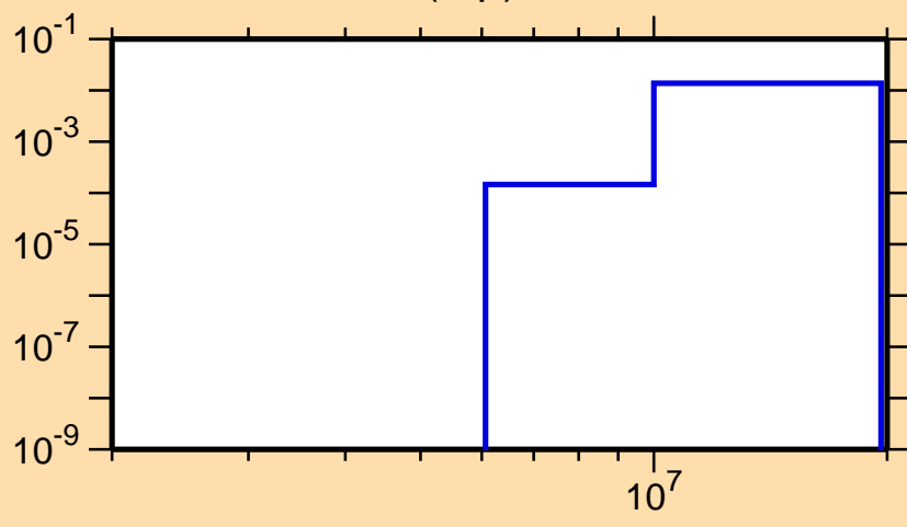
\sigma vs. E for ^{88}\text{Sr}(n,p)
