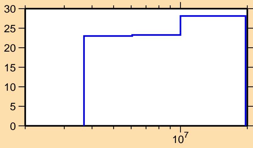
\Delta\sigma/\sigma vs. E for ^{88}\text{Sr}(n,\gamma)
