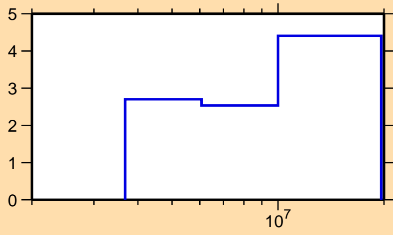
\Delta\sigma/\sigma vs. E for ^{88}\text{Sr}(n,\text{inel.})
