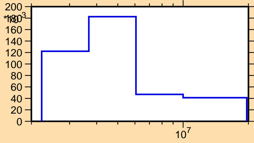
\sigma vs. E for ^{88}\text{Sr}(n,n_2)
