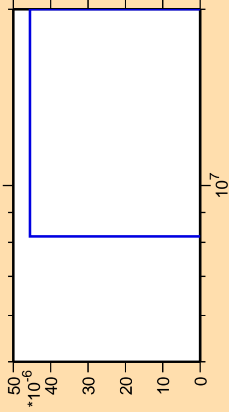
\Delta\sigma/\sigma vs. E for ^{88}\text{Sr}(n,\text{nd})
