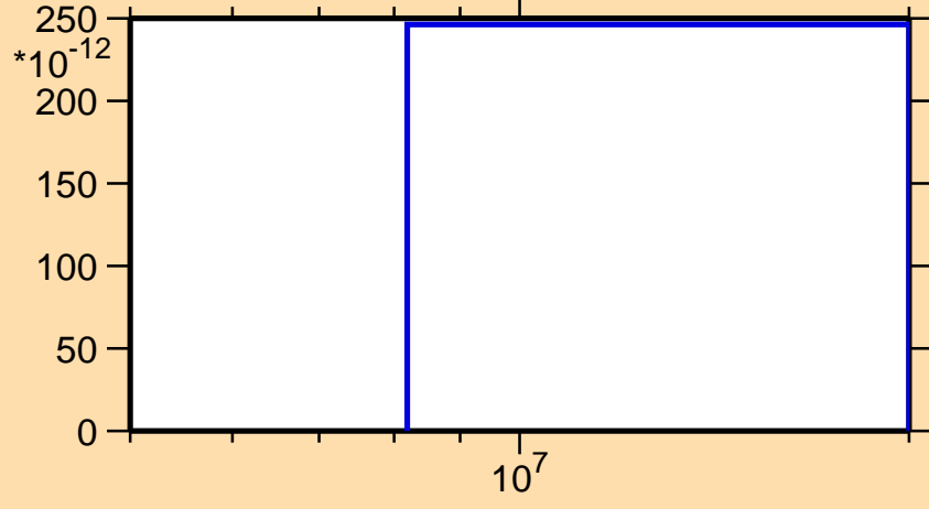
\sigma vs. E for ^{88}\text{Sr}(n,3n)
