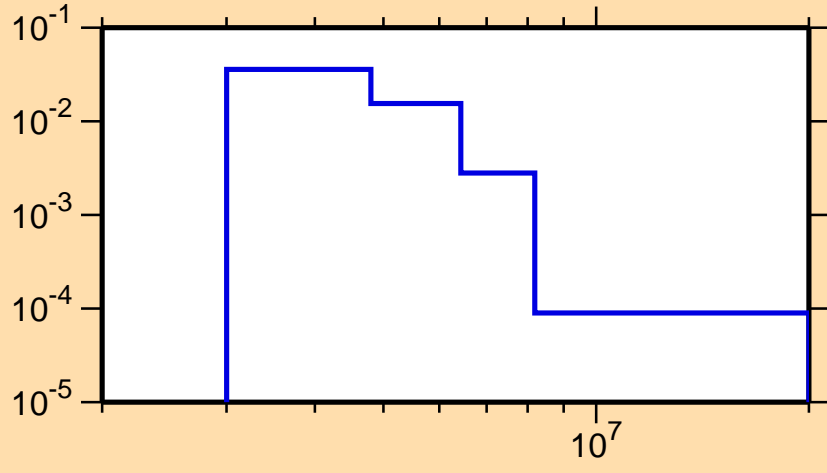
\sigma vs. E for ^{88}\text{Sr}(n,n_3)
