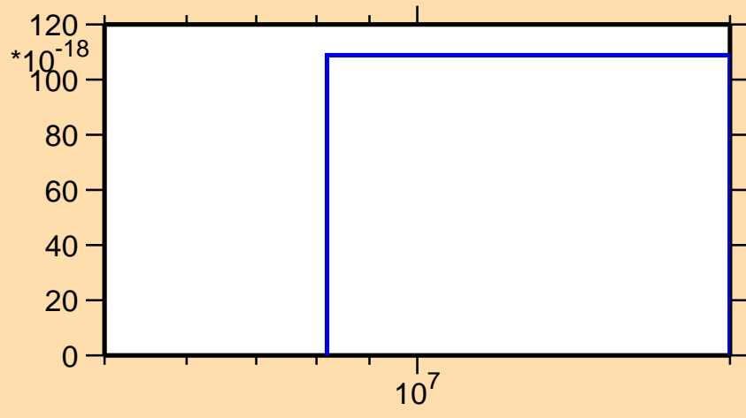
\sigma vs. E for ^{88}\text{Sr}(n,\text{nd})
