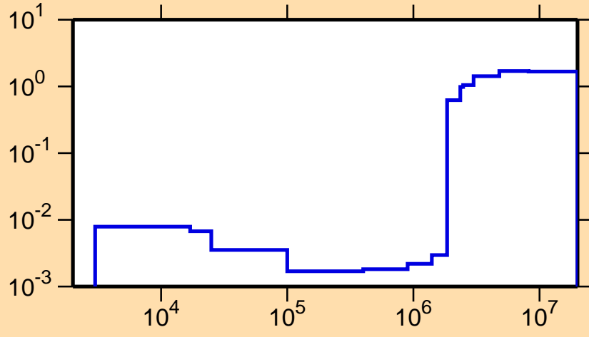
\sigma vs. E for ^{88}\text{Sr}(n,\text{nonel.})
