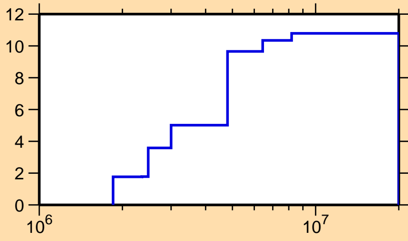
\Delta\sigma/\sigma vs. E for ^{88}\text{Sr}(n,n_1)
