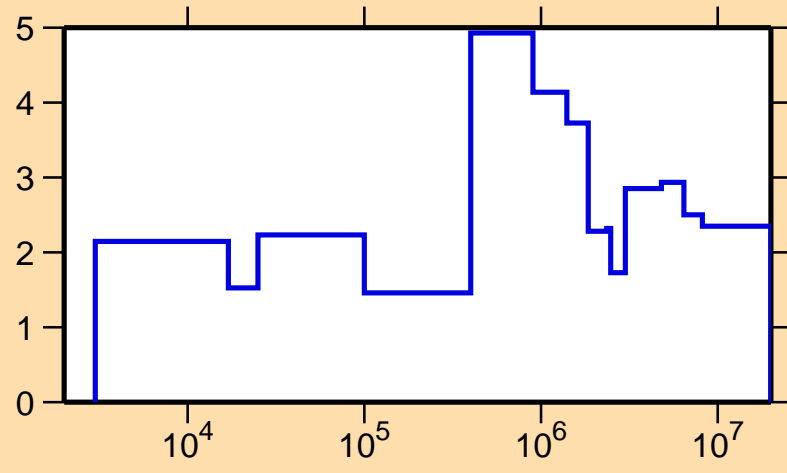
\Delta\sigma/\sigma vs. E for ^{88}\text{Sr}(n,\text{el.})
