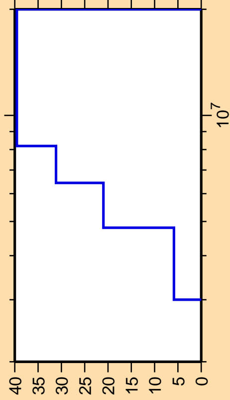
\Delta\sigma/\sigma vs. E for ^{88}\text{Sr}(n,n_3)
