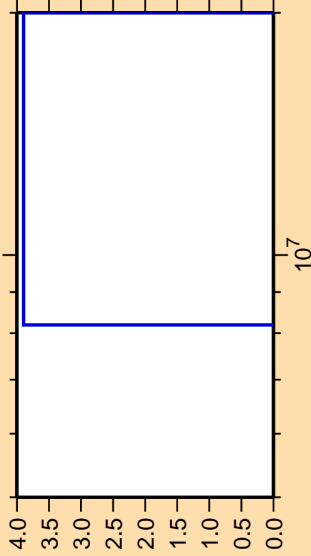
\Delta\sigma/\sigma vs. E for ^{88}\text{Sr}(n,2n)
