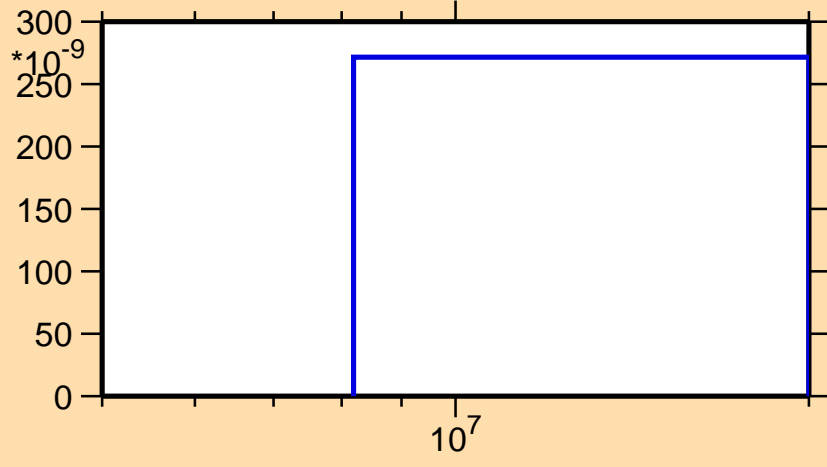
\sigma vs. E for ^{88}\text{Sr}(n,t)
