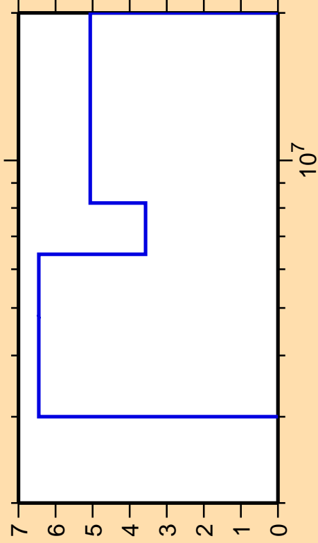
\Delta\sigma/\sigma vs. E for ^{88}\text{Sr}(n,n\text{cont.})
