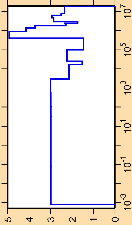
\Delta\sigma/\sigma vs. E for ^{88}\text{Sr}(n,\text{el.})
