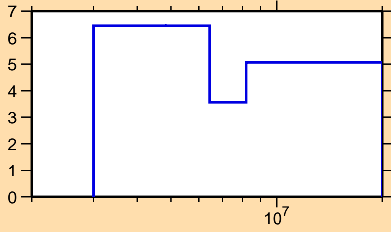
\Delta\sigma/\sigma vs. E for ^{88}\text{Sr}(n,n\text{cont.})
