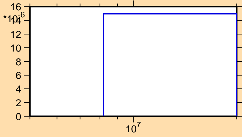
\sigma vs. E for ^{88}\text{Sr}(n,\alpha)
