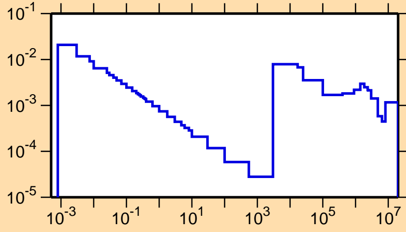
\sigma vs. E for ^{88}\text{Sr}(n,\gamma)
