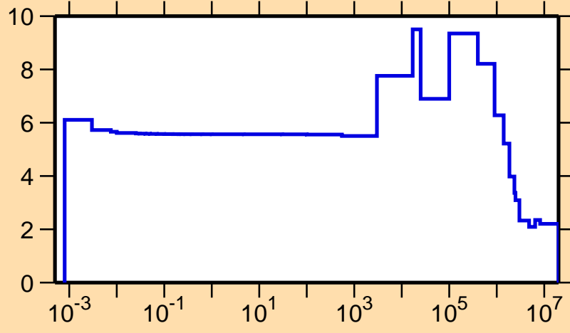
\sigma vs. E for ^{88}\text{Sr}(n,\text{el.})
