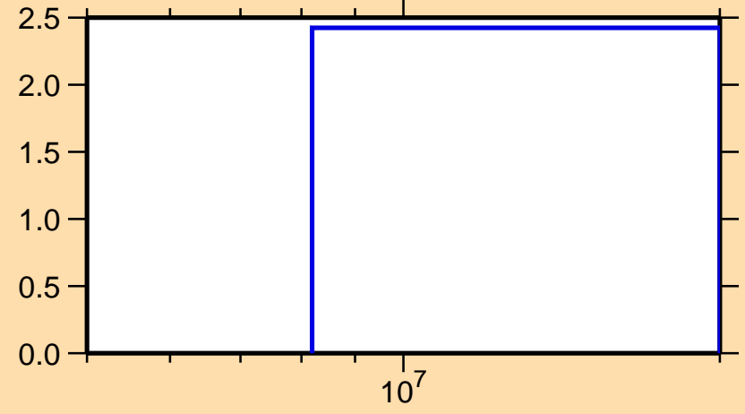
\Delta\sigma/\sigma vs. E for ^{88}\text{Sr}(n,\text{nonel.})
