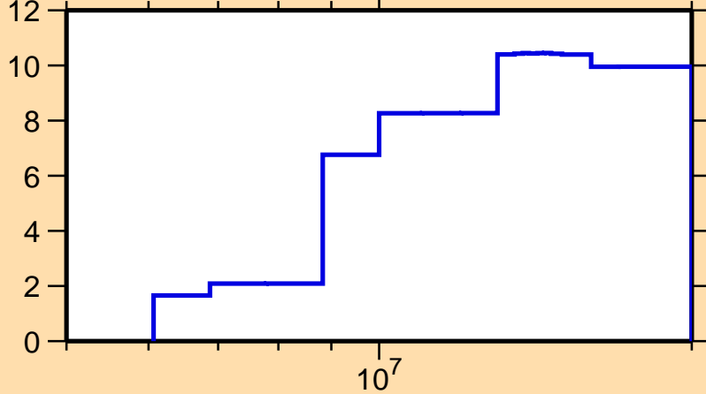
\Delta\sigma/\sigma vs. E for ^{89}\text{Sr}(n,\text{inel.})
