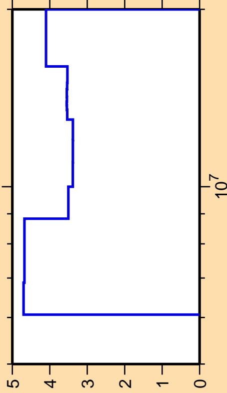
\Delta\sigma/\sigma vs. E for ^{89}\text{Sr}(n,2n)
