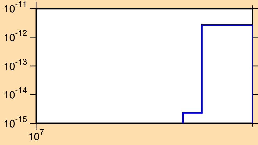
\sigma vs. E for ^{89}\text{Sr}(n,\text{He}3)
