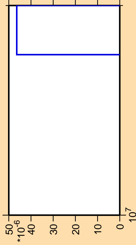
\Delta\sigma/\sigma vs. E for ^{89}\text{Sr}(n,nt)
