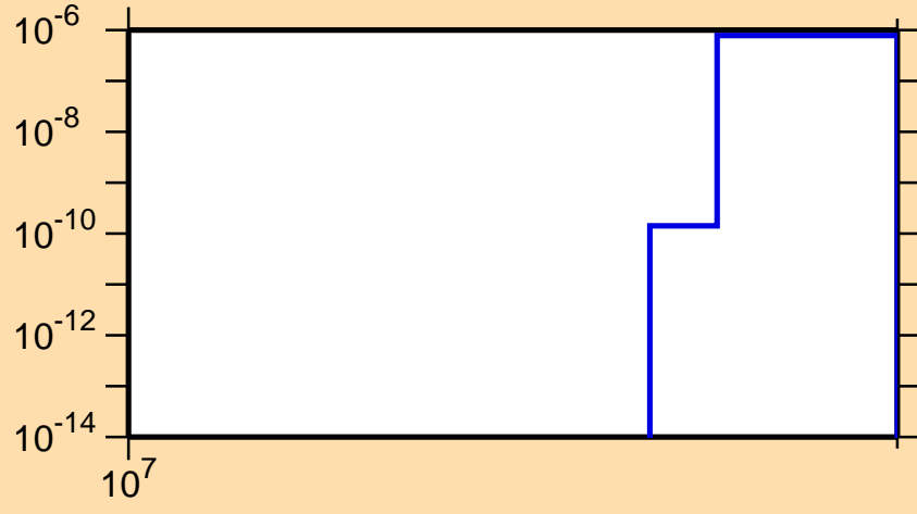
\sigma vs. E for ^{89}\text{Sr}(n,\text{nd})
