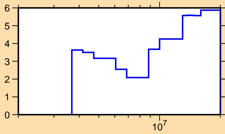
\Delta\sigma/\sigma vs. E for ^{89}\text{Sr}(n,\text{el.})
