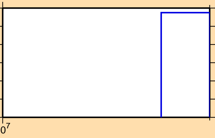
\sigma vs. E for ^{89}\text{Sr}(n,2np)
