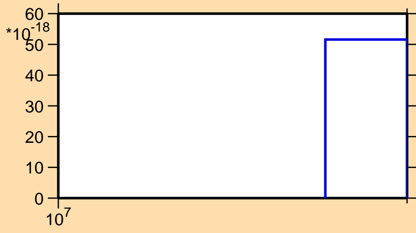
\sigma vs. E for ^{89}\text{Sr}(n,nt)
