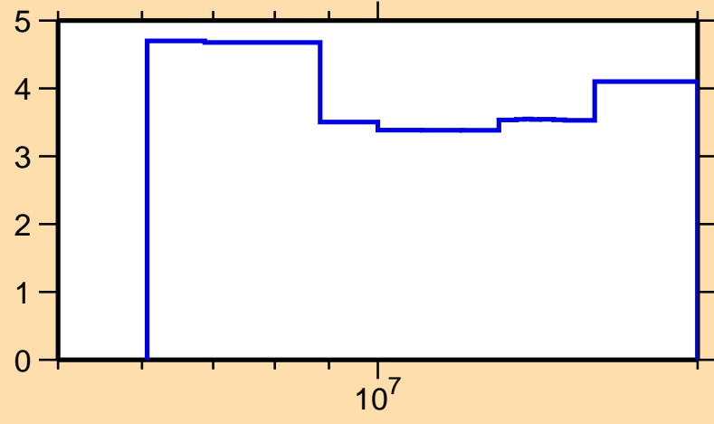
\Delta\sigma/\sigma vs. E for ^{89}\text{Sr}(n,2n)
