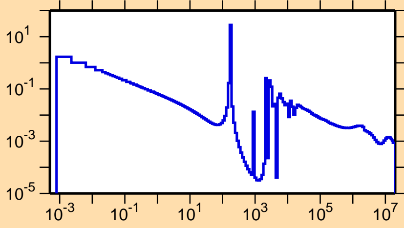
\sigma vs. E for ^{89}\text{Sr}(n,\gamma)
