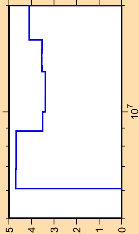
\Delta\sigma/\sigma vs. E for ^{89}\text{Sr}(n,2n)
