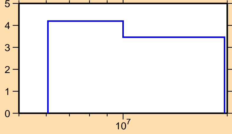
\Delta\sigma/\sigma vs. E for ^{89}\text{Sr}(n,2n)
