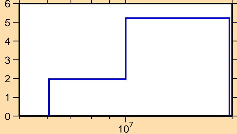
\Delta\sigma/\sigma vs. E for ^{89}\text{Sr}(n,\text{el.})
