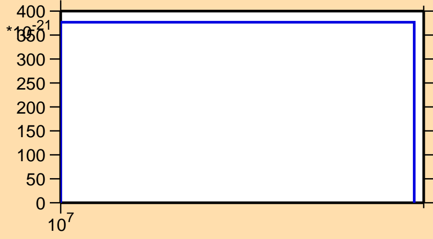
\sigma vs. E for ^{89}\text{Sr}(n,nt)
