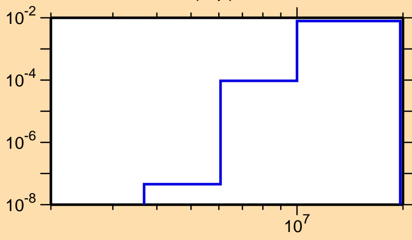
\sigma vs. E for ^{89}\text{Sr}(n,p)
