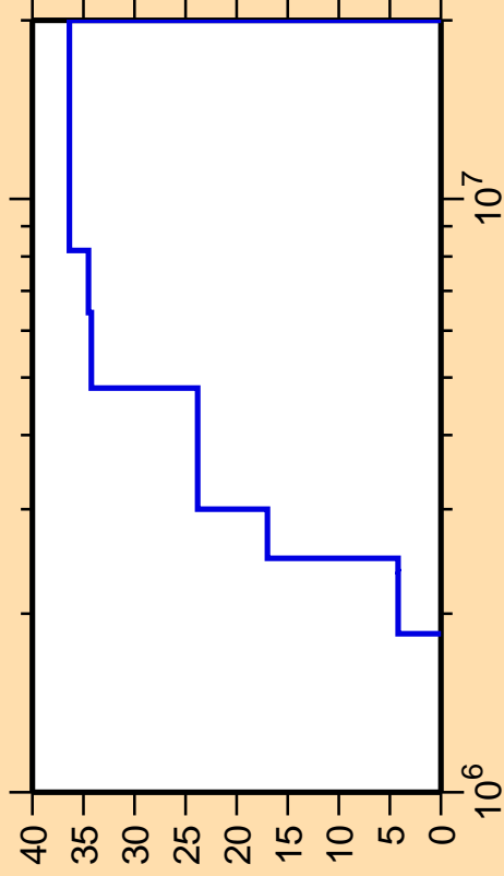
\Delta\sigma/\sigma vs. E for ^{89}\text{Sr}(n,n_3)
