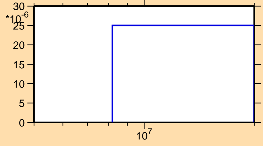
\sigma vs. E for ^{89}\text{Sr}(n,3n)
