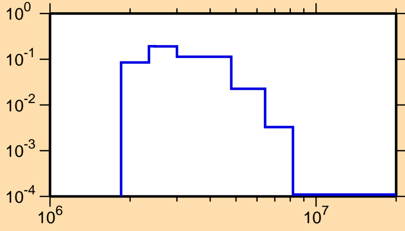
\sigma vs. E for ^{89}\text{Sr}(n,n_3)
