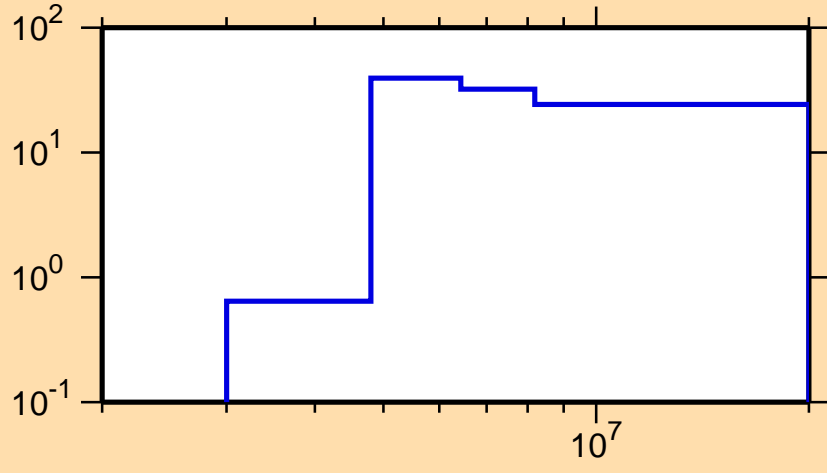
\Delta\sigma/\sigma vs. E for ^{89}\text{Sr}(n,p)
