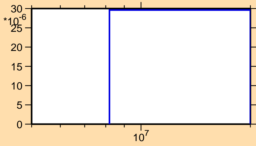
\sigma vs. E for ^{89}\text{Sr}(n,n\alpha)
