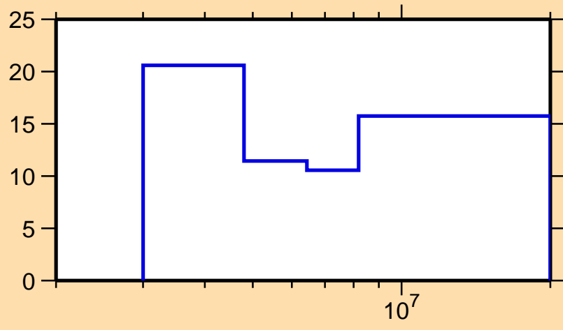
\Delta\sigma/\sigma vs. E for ^{89}\text{Sr}(n,n_1)
