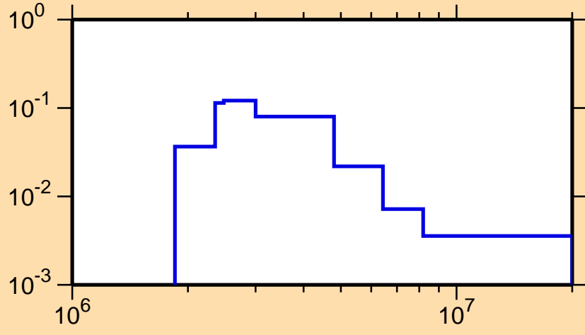
\sigma vs. E for ^{89}\text{Sr}(n,n_4)
