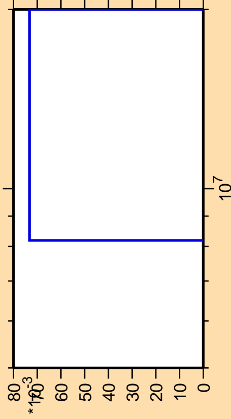
\Delta\sigma/\sigma vs. E for ^{89}\text{Sr}(n,\text{He}3)
