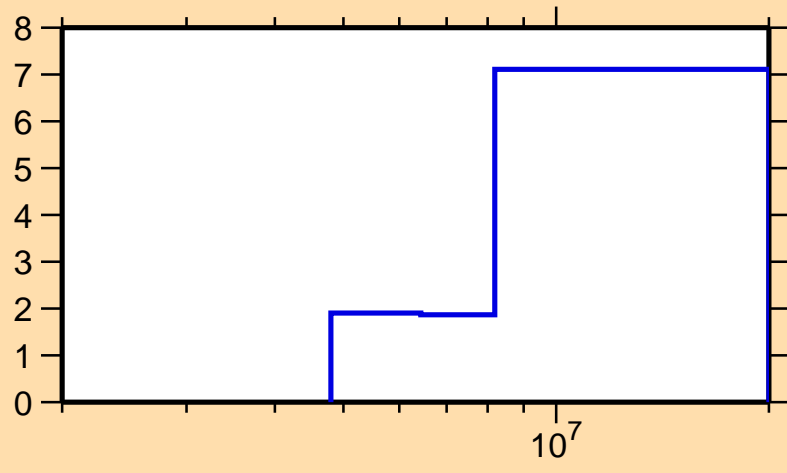
\Delta\sigma/\sigma vs. E for ^{89}\text{Sr}(n,\text{inel.})
