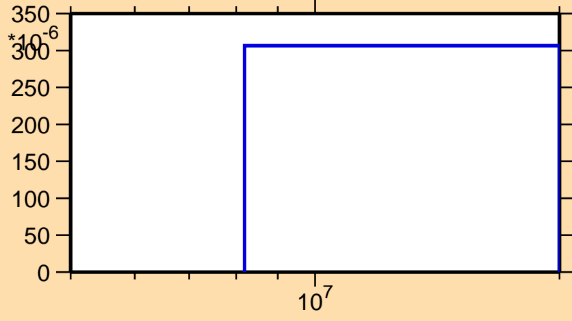
\sigma vs. E for ^{89}\text{Sr}(n,d)
