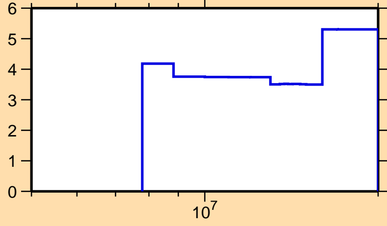
\Delta\sigma/\sigma vs. E for ^{90}\text{Sr}(n,2n)
