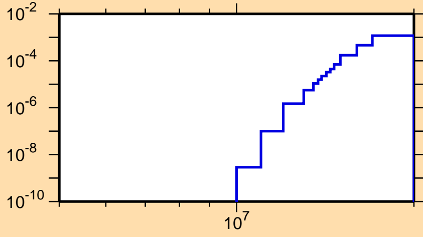
\sigma vs. E for ^{90}\text{Sr}(n,\alpha)
