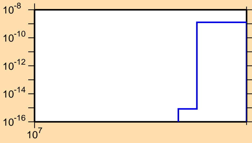
\sigma vs. E for ^{90}\text{Sr}(n,nt)
