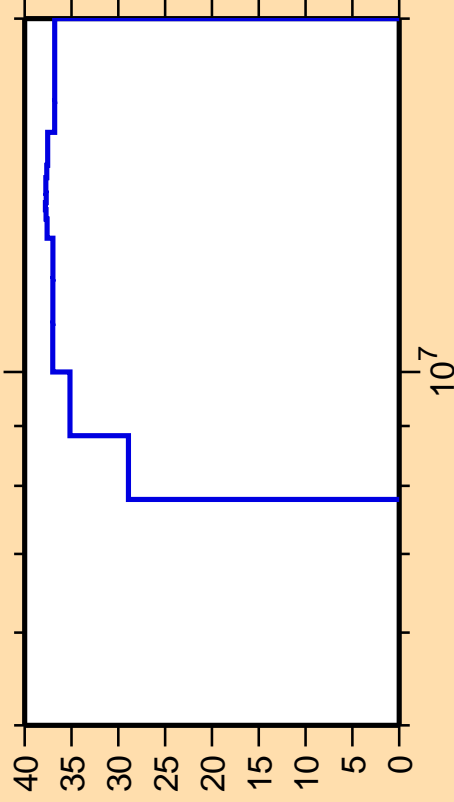
\Delta\sigma/\sigma vs. E for ^{90}\text{Sr}(n,\gamma)
