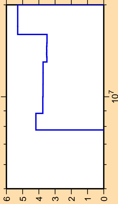
\Delta\sigma/\sigma vs. E for ^{90}\text{Sr}(n,2n)
