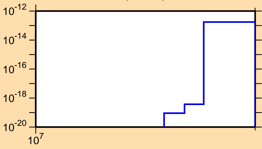
\sigma vs. E for ^{90}\text{Sr}(n,2n\alpha)
