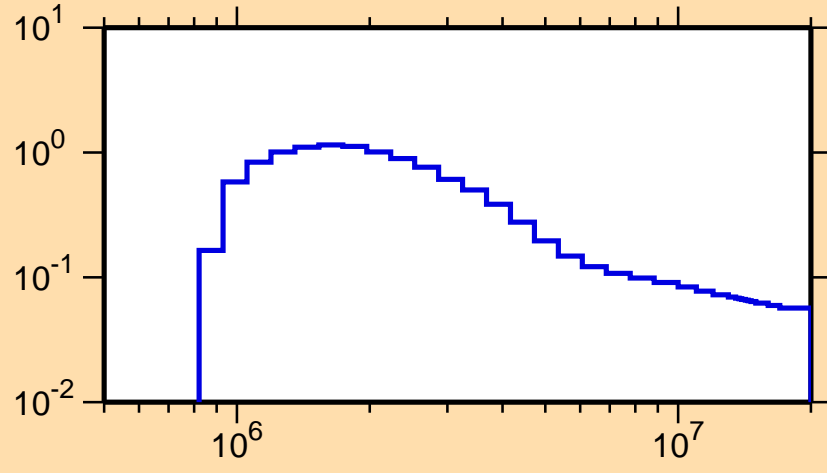
\sigma vs. E for ^{90}\text{Sr}(n,n_1)
