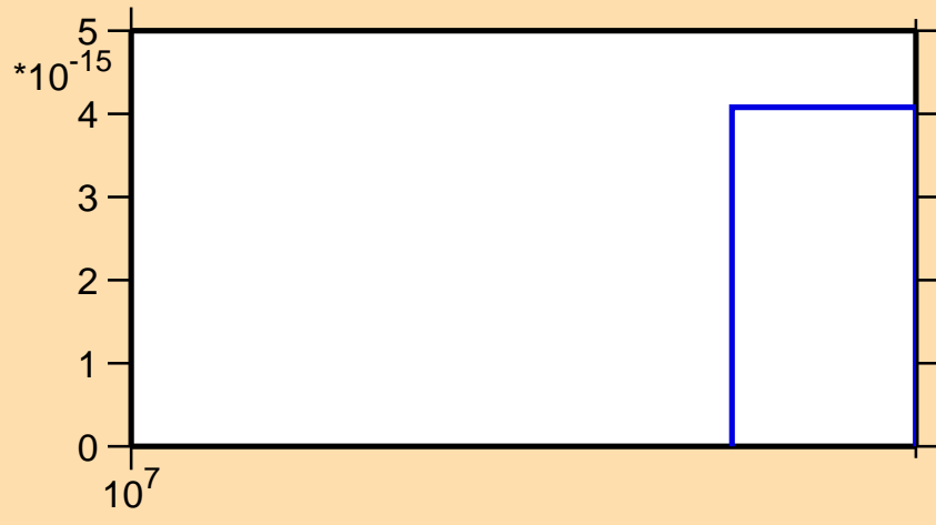
\sigma vs. E for ^{90}\text{Sr}(n,2np)
