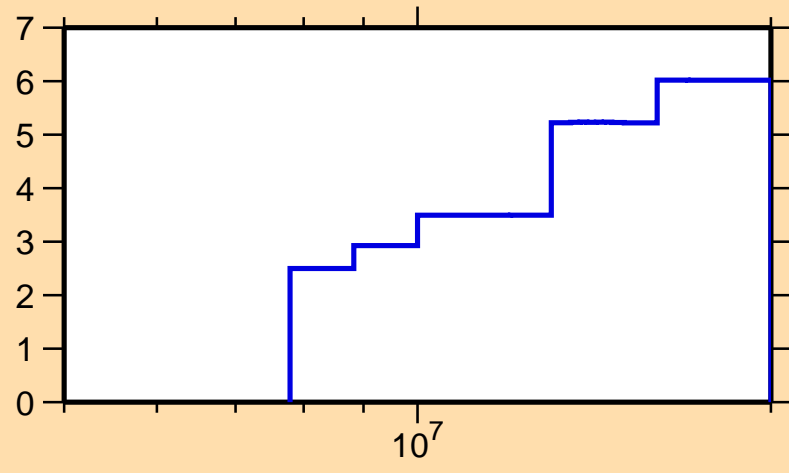
\Delta\sigma/\sigma vs. E for ^{90}\text{Sr}(n,\text{el.})
