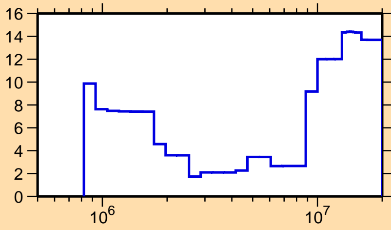
\Delta\sigma/\sigma vs. E for ^{90}\text{Sr}(n,\text{inel.})
