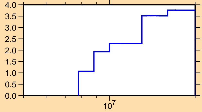
\Delta\sigma/\sigma vs. E for ^{90}\text{Sr}(n,\text{tot.})
