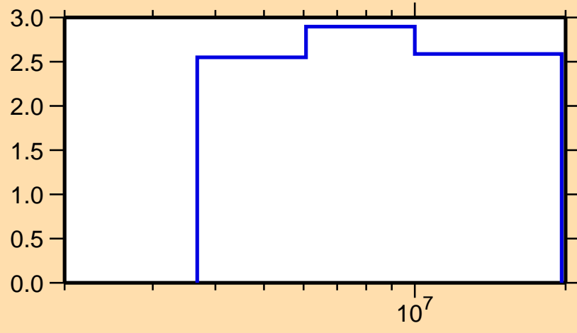
\Delta\sigma/\sigma vs. E for ^{90}\text{Sr}(n,n\text{onel.})
