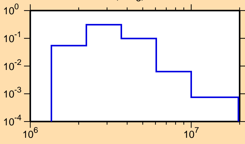
\sigma vs. E for ^{90}\text{Sr}(n,n_3)
