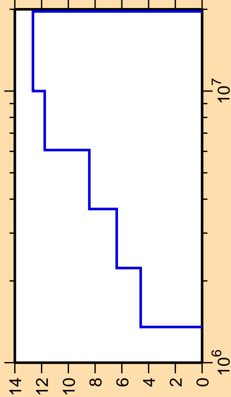
\Delta\sigma/\sigma vs. E for ^{90}\text{Sr}(n,n_2)
