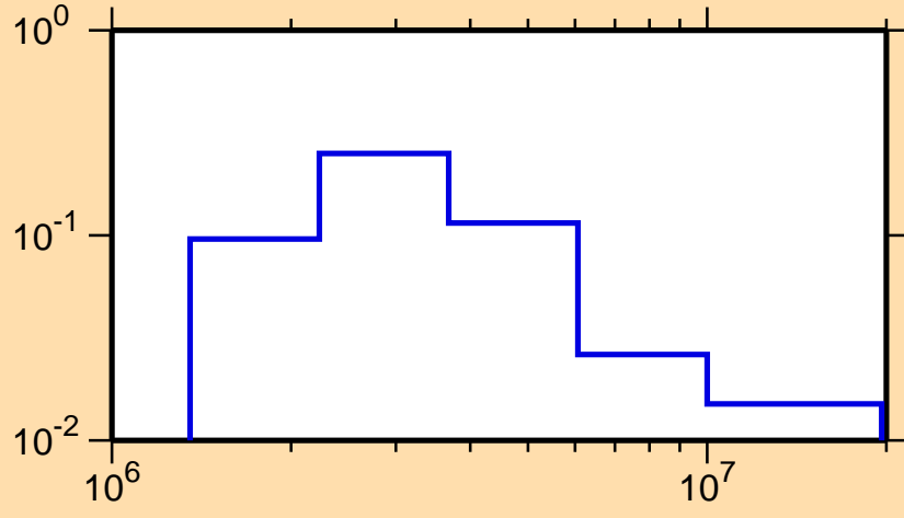
\sigma vs. E for ^{90}\text{Sr}(n,n_2)
