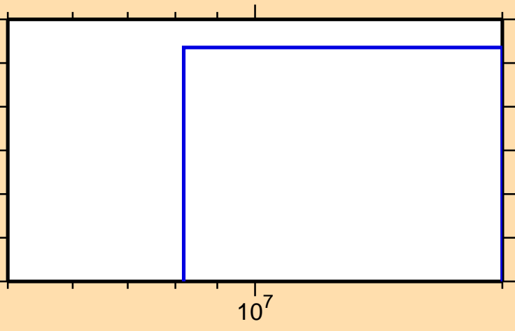
\sigma vs. E for ^{90}\text{Sr}(n,\text{He}3)
