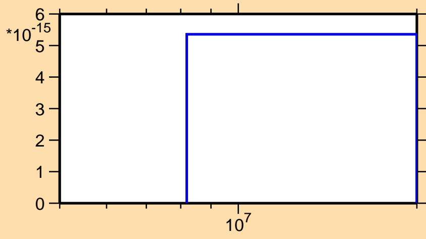
\sigma vs. E for ^{90}\text{Sr}(n,\text{He}3)
