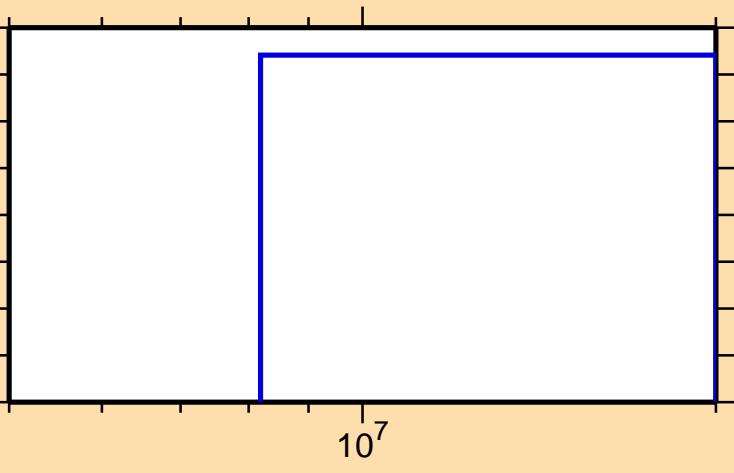
\sigma vs. E for ^{90}\text{Sr}(n,d)
