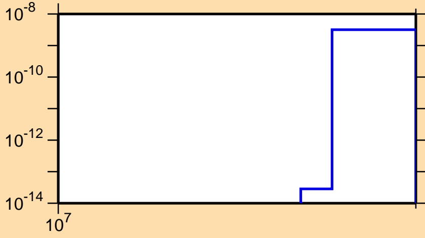
\sigma vs. E for ^{92}\text{Sr}(n,nt)
