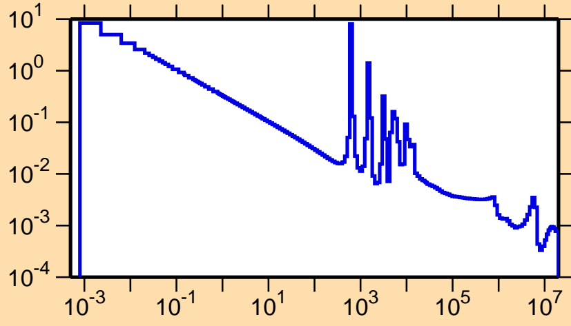
\sigma vs. E for ^{92}\text{Sr}(n,\gamma)
