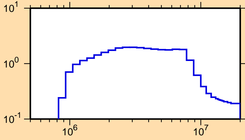
\sigma vs. E for ^{92}\text{Sr}(n,\text{inel.})
