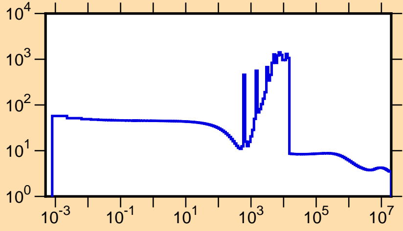
\sigma vs. E for ^{92}\text{Sr}(n,\text{tot.})
