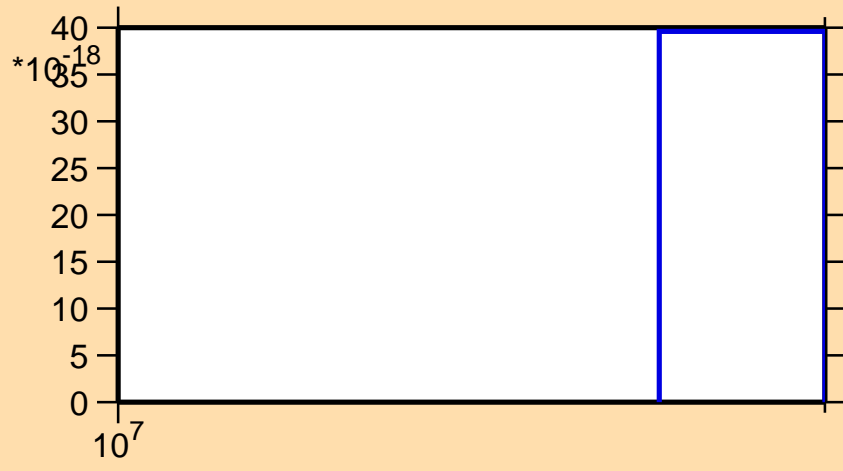
\sigma vs. E for ^{92}\text{Sr}(n,2np)
