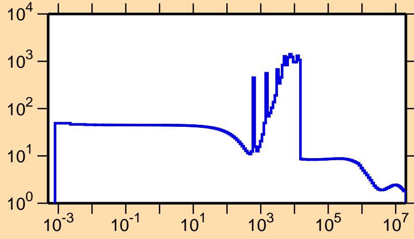
\sigma vs. E for ^{92}\text{Sr}(n,\text{el.})
