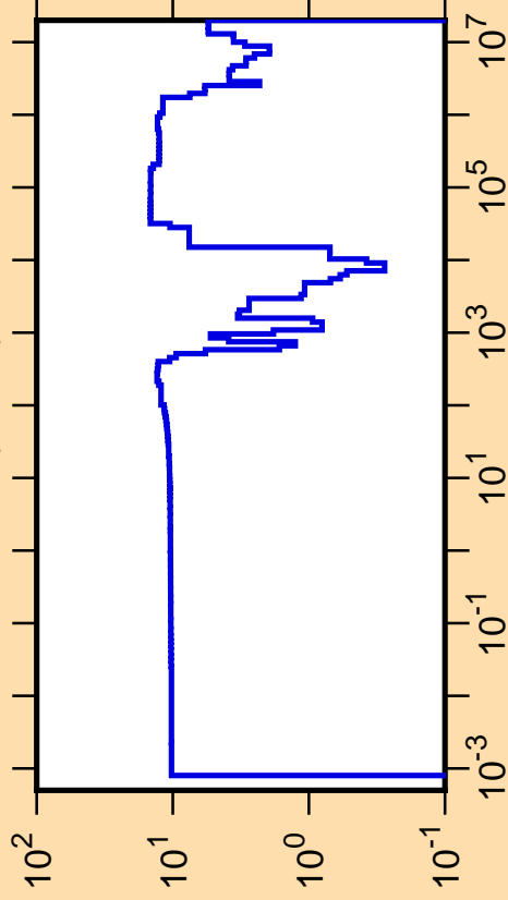
\Delta\sigma/\sigma vs. E for ^{92}\text{Sr}(n,\text{tot.})
