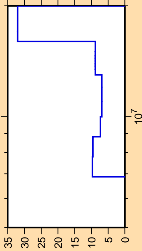
\Delta\sigma/\sigma vs. E for ^{92}\text{Sr}(n,2n)
