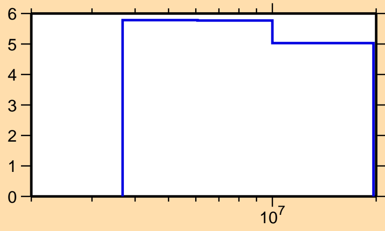
\Delta\sigma/\sigma vs. E for ^{92}\text{Sr}(n,\text{nonel.})
