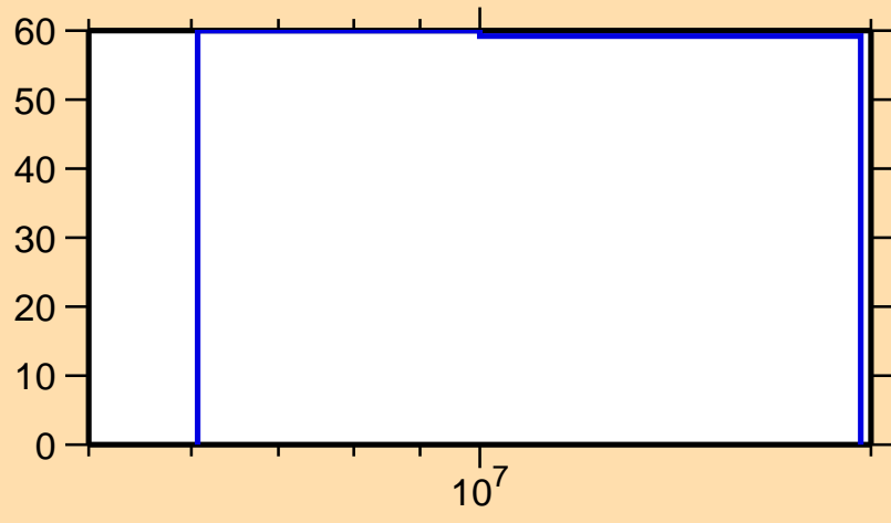
\Delta\sigma/\sigma vs. E for ^{92}\text{Sr}(n,p)
