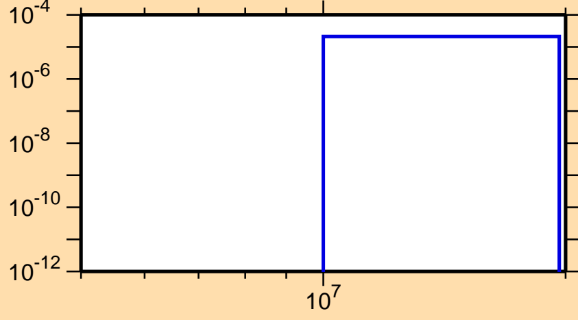
\sigma vs. E for ^{92}\text{Sr}(n,\alpha)
