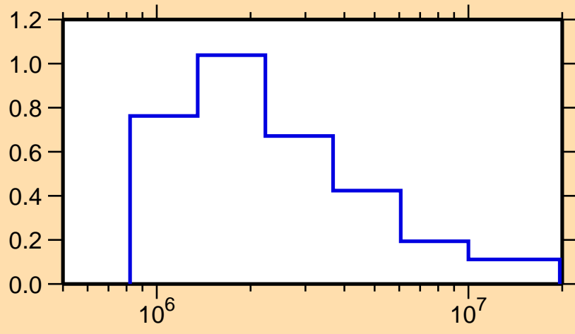
\sigma vs. E for ^{92}\text{Sr}(n,n_1)
