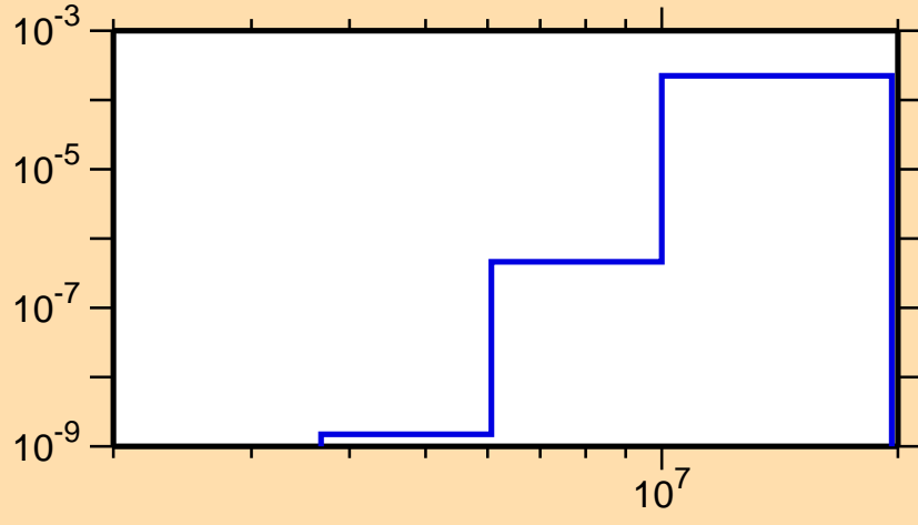
\sigma vs. E for ^{92}\text{Sr}(n,\alpha)
