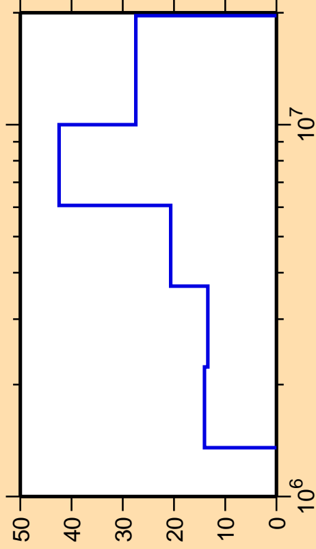
\Delta\sigma/\sigma vs. E for ^{92}\text{Sr}(n,n_4)
