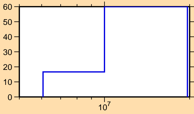
\Delta\sigma/\sigma vs. E for ^{92}\text{Sr}(n,ncont.)
