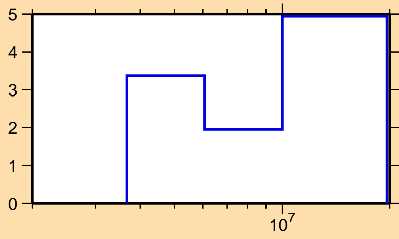
\Delta\sigma/\sigma vs. E for ^{92}\text{Sr}(n,\text{tot.})
