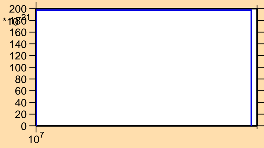
\sigma vs. E for ^{92}\text{Sr}(n,2np)
