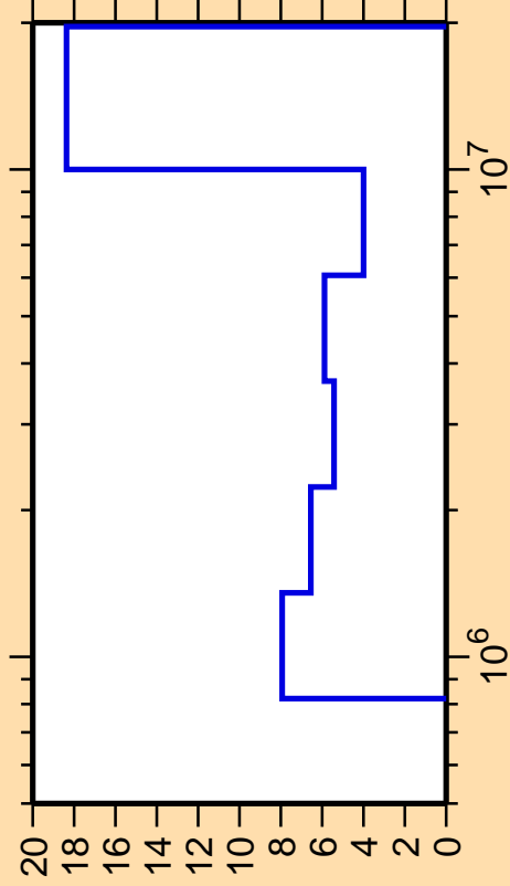
\Delta\sigma/\sigma vs. E for ^{92}\text{Sr}(n,\text{inel.})
