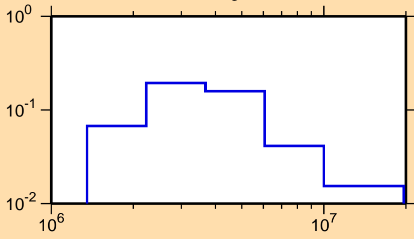
\sigma vs. E for ^{92}\text{Sr}(n,n_3)
