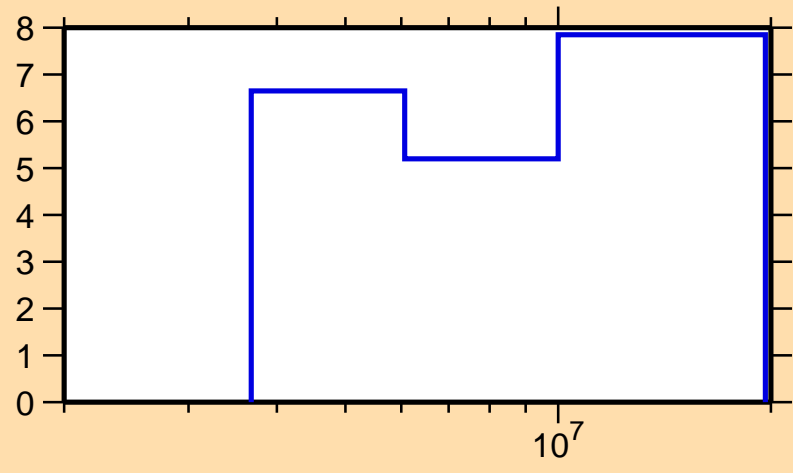
\Delta\sigma/\sigma vs. E for ^{92}\text{Sr}(n,\text{el.})
