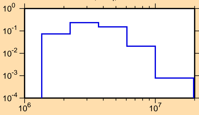
\sigma vs. E for ^{92}\text{Sr}(n,n_4)
