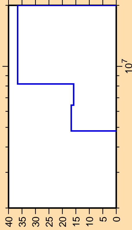
\Delta\sigma/\sigma vs. E for ^{92}\text{Sr}(n,ncont.)
