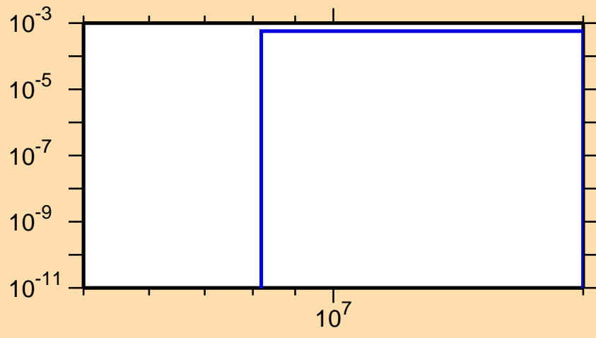
\sigma vs. E for ^{92}\text{Sr}(n,p)
