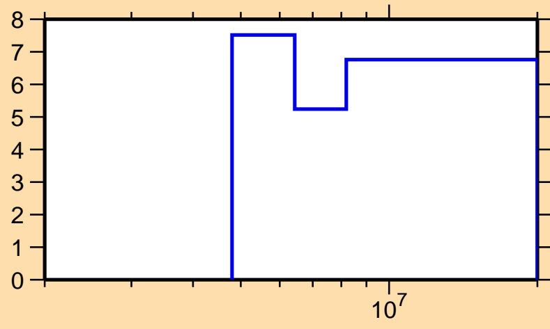
\Delta\sigma/\sigma vs. E for ^{92}\text{Sr}(n,el.)
