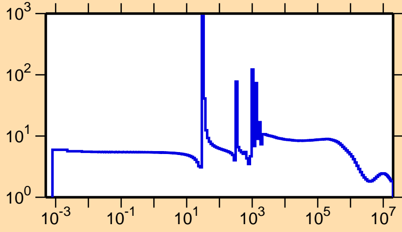
\sigma vs. E for ^{93}\text{Sr}(n,\text{el.})
