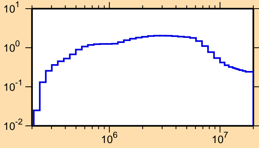
\sigma vs. E for ^{93}\text{Sr}(n,\text{inel.})
