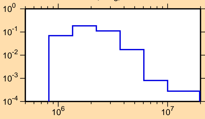
\sigma vs. E for ^{93}\text{Sr}(n,n_3)
