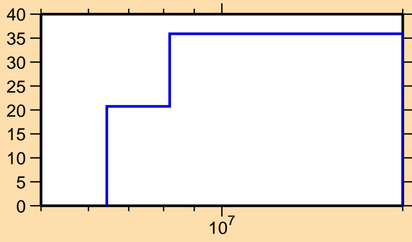
\Delta\sigma/\sigma vs. E for ^{93}\text{Sr}(n,ncont.)
