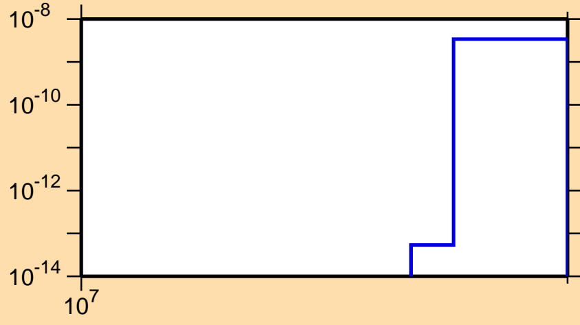
\sigma vs. E for ^{94}\text{Sr}(n,nt)
