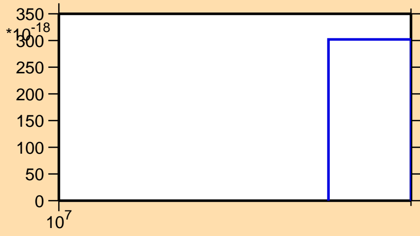
\sigma vs. E for ^{94}\text{Sr}(n,2np)
