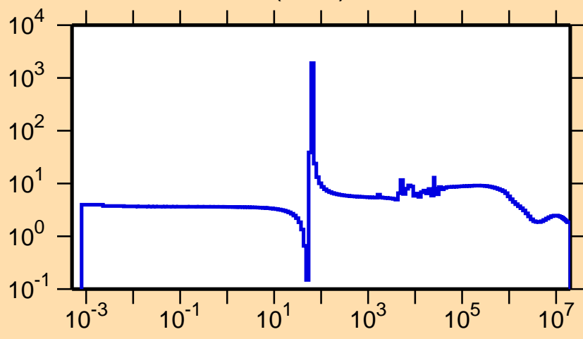
\sigma vs. E for ^{94}\text{Sr}(n,\text{el.})
