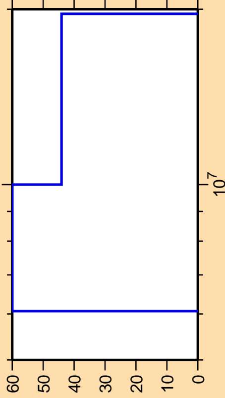
\Delta\sigma/\sigma vs. E for ^{94}\text{Sr}(n,n_1)
