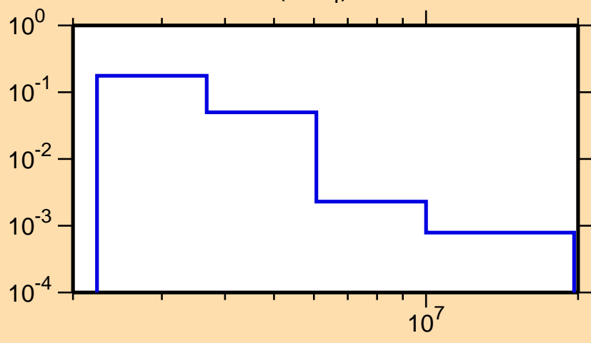
\sigma vs. E for ^{94}\text{Sr}(n,n_4)
