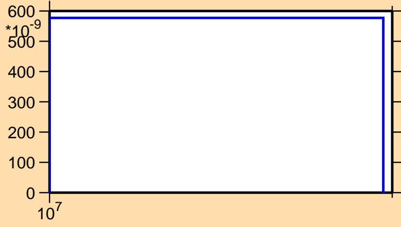
\sigma vs. E for ^{94}\text{Sr}(n,np)
