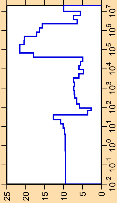
\Delta\sigma/\sigma vs. E for ^{94}\text{Sr}(n,\text{el.})
