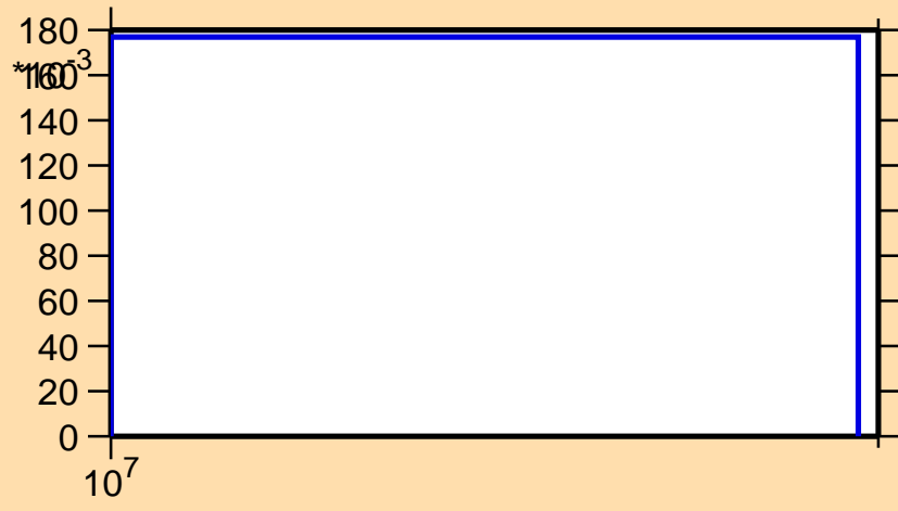
\sigma vs. E for ^{94}\text{Sr}(n,3n)
