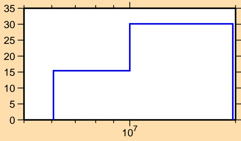
\Delta\sigma/\sigma vs. E for ^{94}\text{Sr}(n,\text{inel.})
