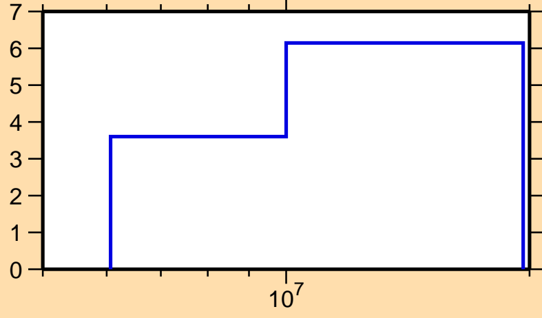
\Delta\sigma/\sigma vs. E for ^{94}\text{Sr}(n,\text{tot.})
