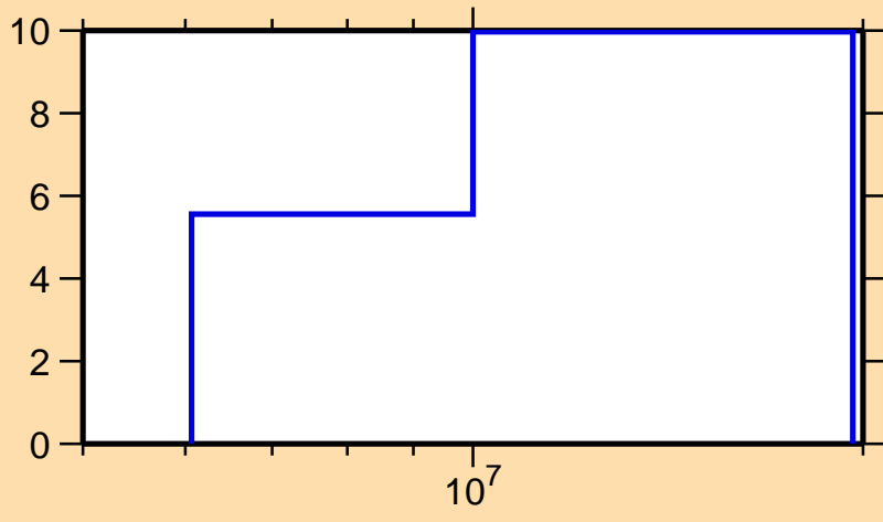
\Delta\sigma/\sigma vs. E for ^{94}\text{Sr}(n,\text{el.})
