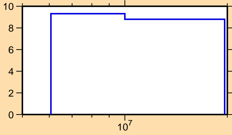
\Delta\sigma/\sigma vs. E for ^{94}\text{Sr}(n,\text{nonel.})
