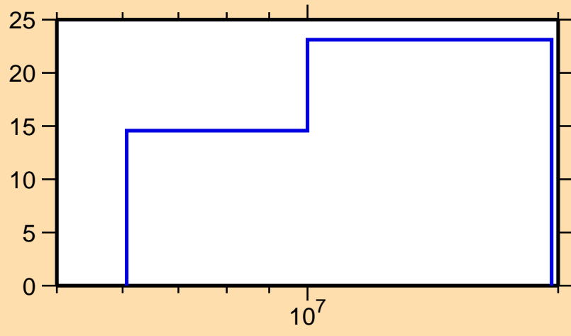
\Delta\sigma/\sigma vs. E for ^{94}\text{Sr}(n,2n)
