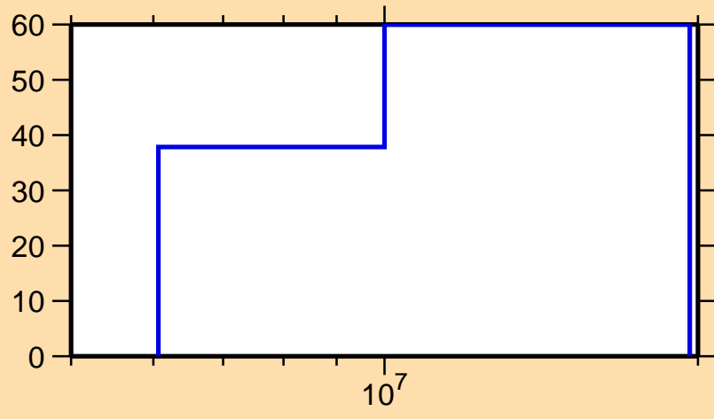
\Delta\sigma/\sigma vs. E for ^{94}\text{Sr}(n,n\text{cont.})
