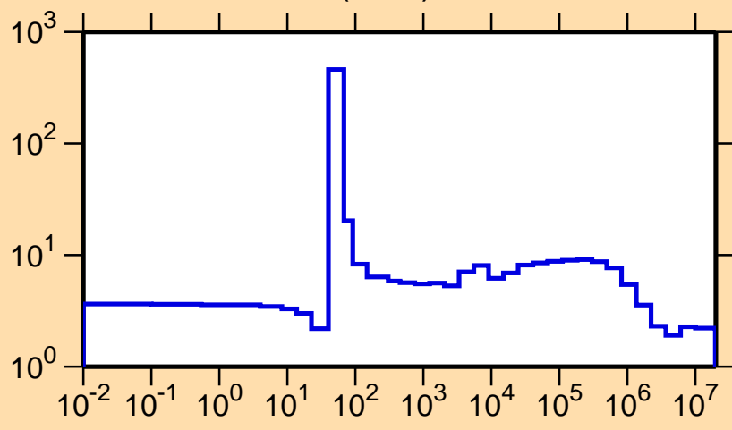
\sigma vs. E for ^{94}\text{Sr}(n,\text{el.})
