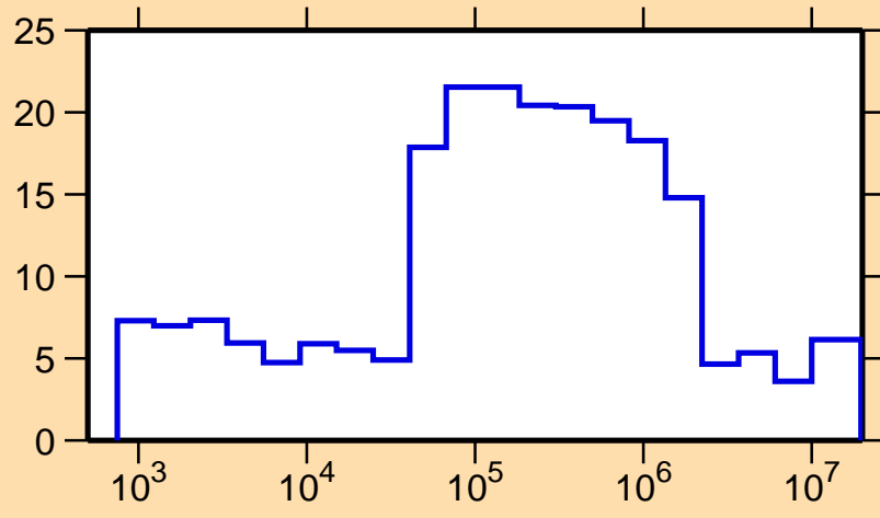
\Delta\sigma/\sigma vs. E for ^{94}\text{Sr}(n,\text{tot.})
