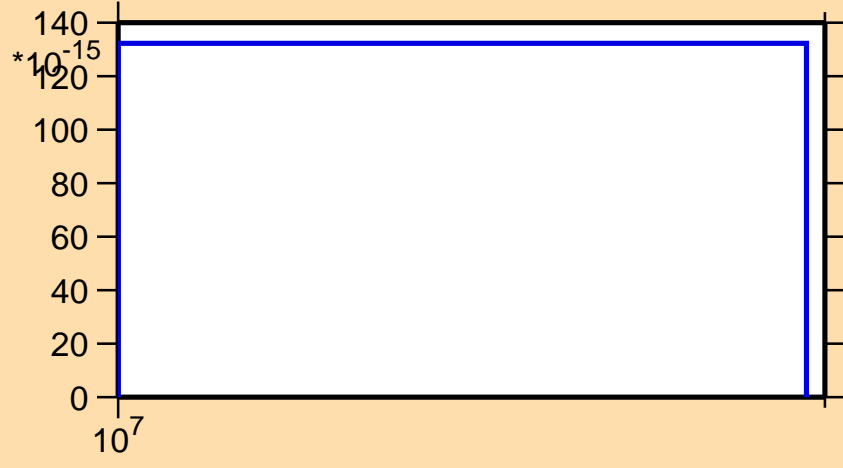
\sigma vs. E for ^{94}\text{Sr}(n,\text{nd})
