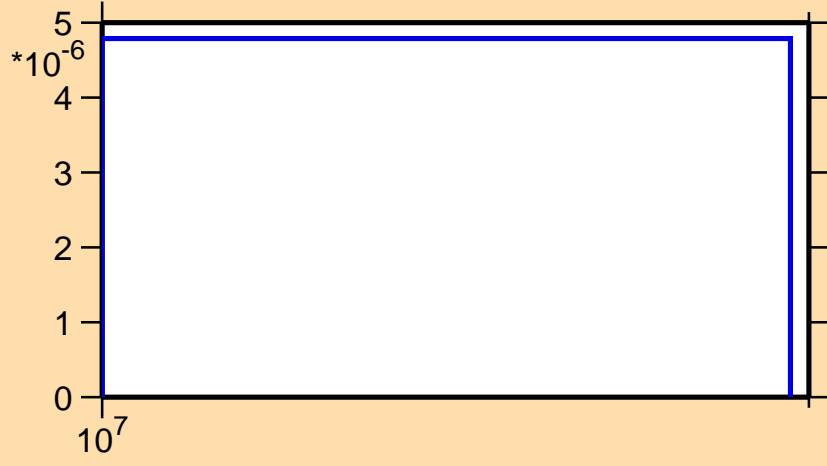
\sigma vs. E for ^{94}\text{Sr}(n,d)
