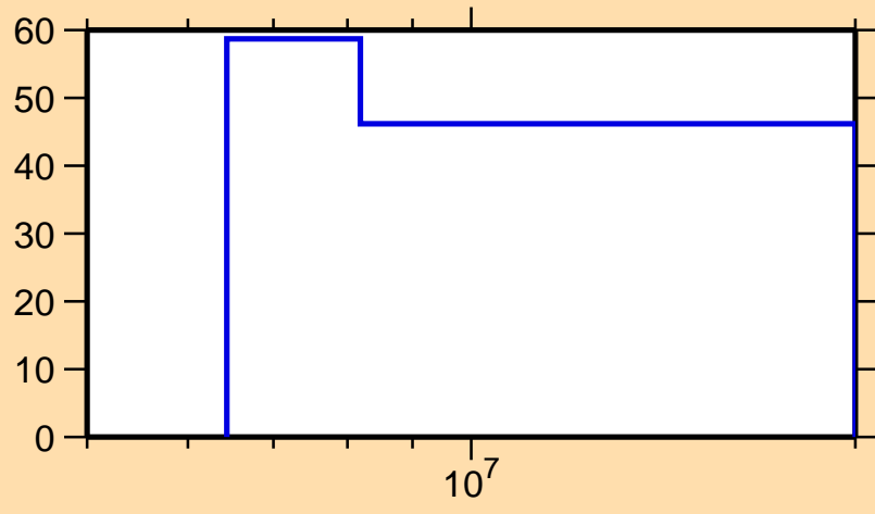
\Delta\sigma/\sigma vs. E for ^{94}\text{Sr}(n,n_1)
