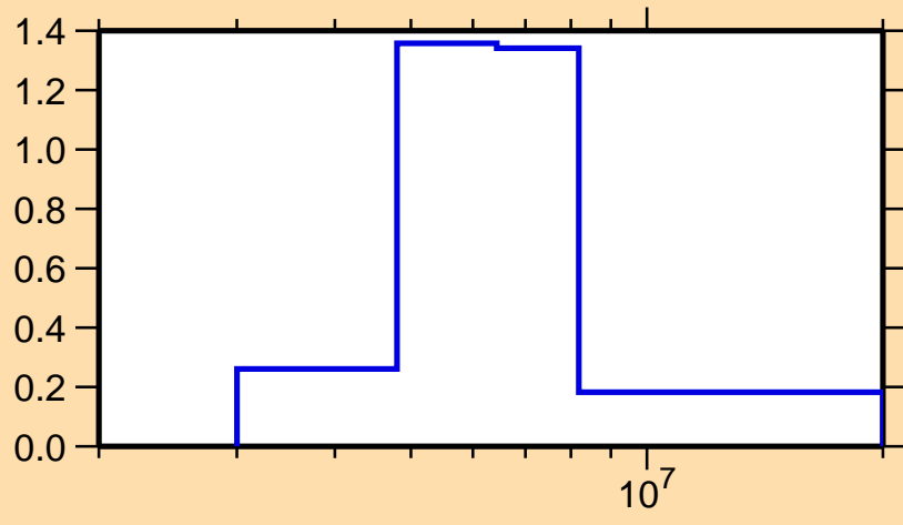
\sigma vs. E for ^{94}\text{Sr}(n,n\text{cont.})
