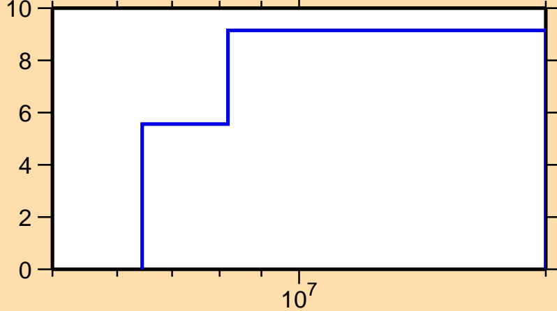
\Delta\sigma/\sigma vs. E for ^{94}\text{Sr}(n,\text{el.})
