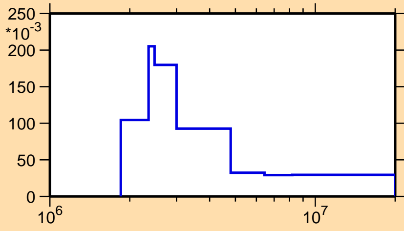
\sigma vs. E for ^{94}\text{Sr}(n,n_2)
