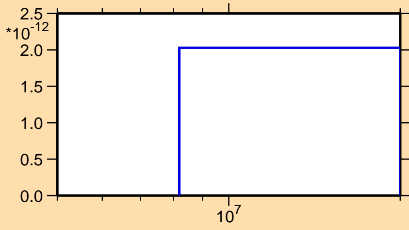
\sigma vs. E for ^{94}\text{Sr}(n,2n\alpha)
