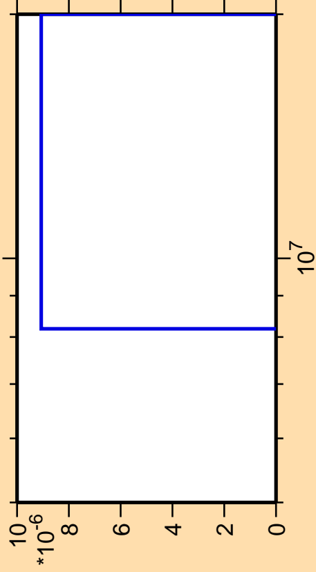
\Delta\sigma/\sigma vs. E for ^{94}\text{Sr}(n,2np)
