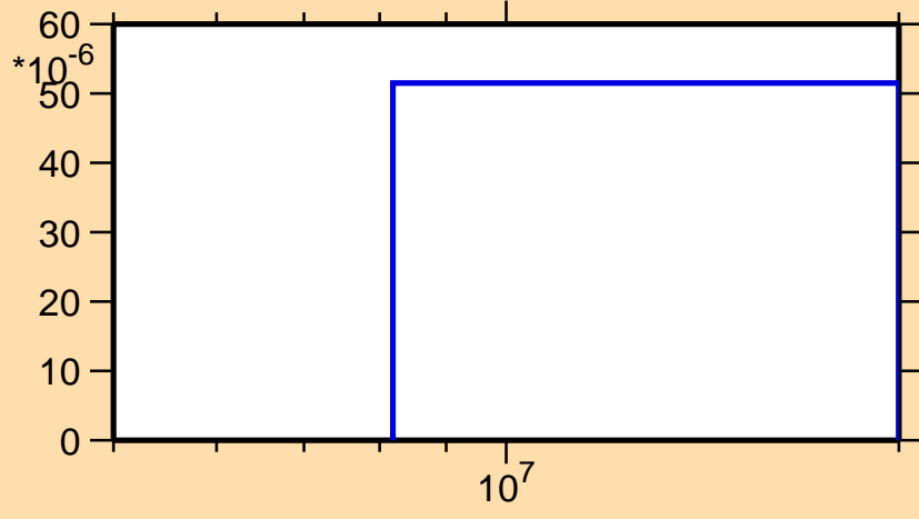
\sigma vs. E for ^{94}\text{Sr}(n,p)
