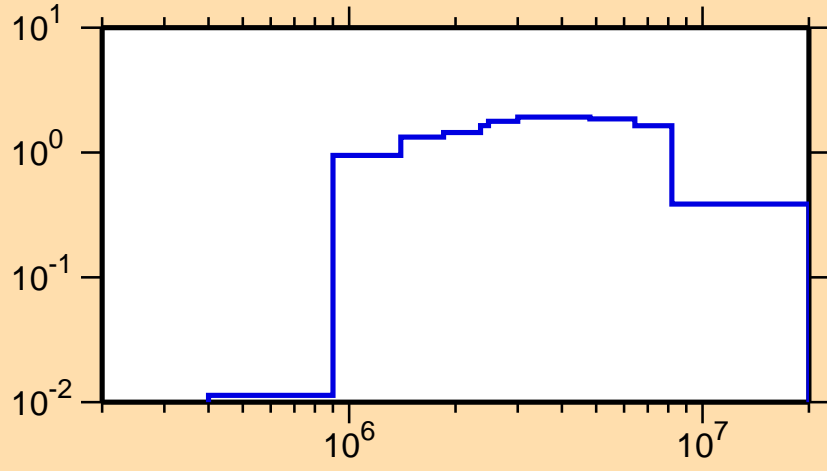
\sigma vs. E for ^{94}\text{Sr}(n,\text{inel.})
