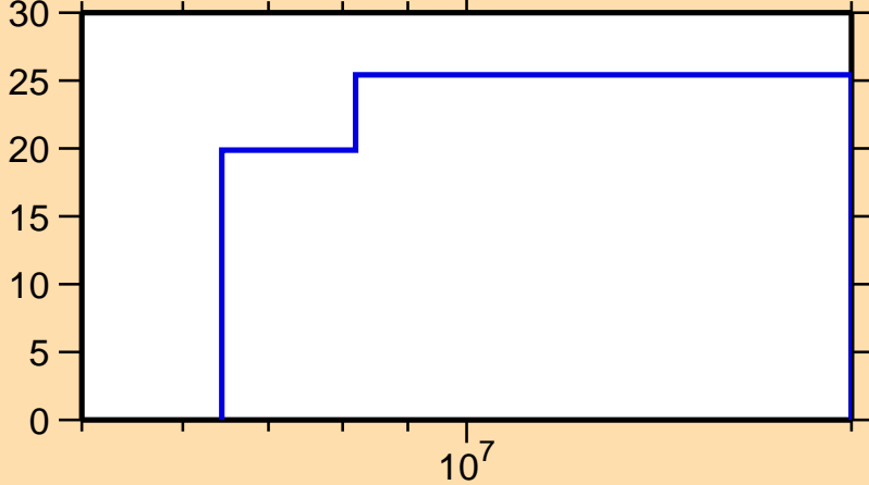
\Delta\sigma/\sigma vs. E for ^{94}\text{Sr}(n,\text{inel.})
