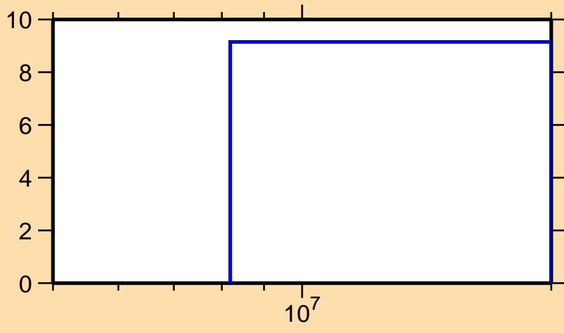
\Delta\sigma/\sigma vs. E for ^{94}\text{Sr}(n,el.)
