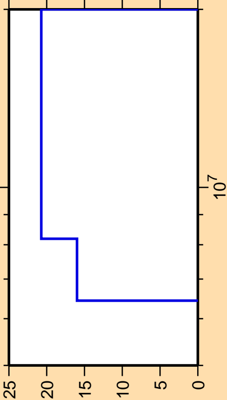
\Delta\sigma/\sigma vs. E for ^{94}\text{Sr}(n,2n)
