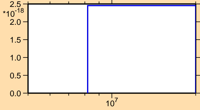
\sigma vs. E for ^{94}\text{Sr}(n,2np)
