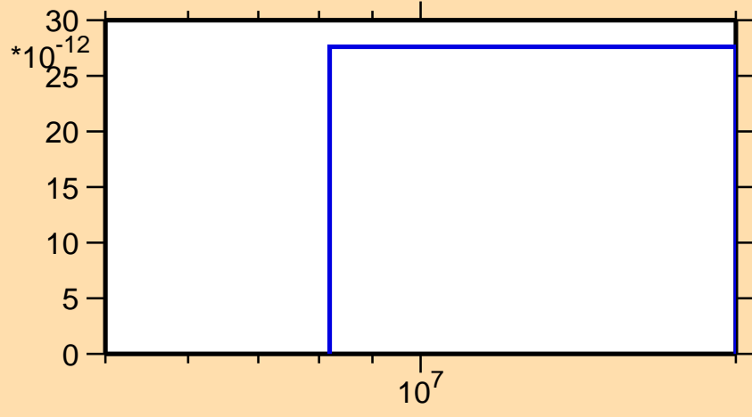
\sigma vs. E for ^{94}\text{Sr}(n,nt)
