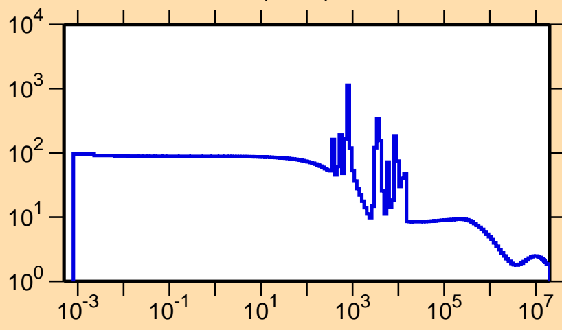
\sigma vs. E for ^{95}\text{Sr}(n,\text{el.})
