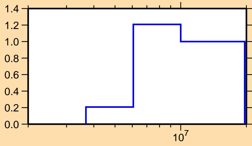
\sigma vs. E for ^{95}\text{Sr}(n,2n)
