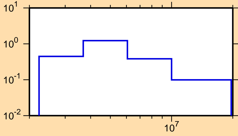
\sigma vs. E for ^{95}\text{Sr}(n,n\text{cont.})
