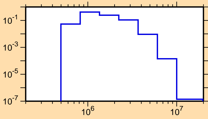
\sigma vs. E for ^{95}\text{Sr}(n,n_3)
