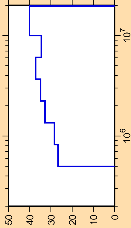
\Delta\sigma/\sigma vs. E for ^{95}\text{Sr}(n,n_3)
