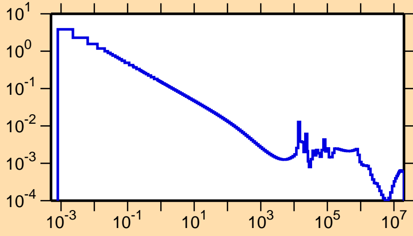
\sigma vs. E for ^{96}\text{Sr}(n,\gamma)
