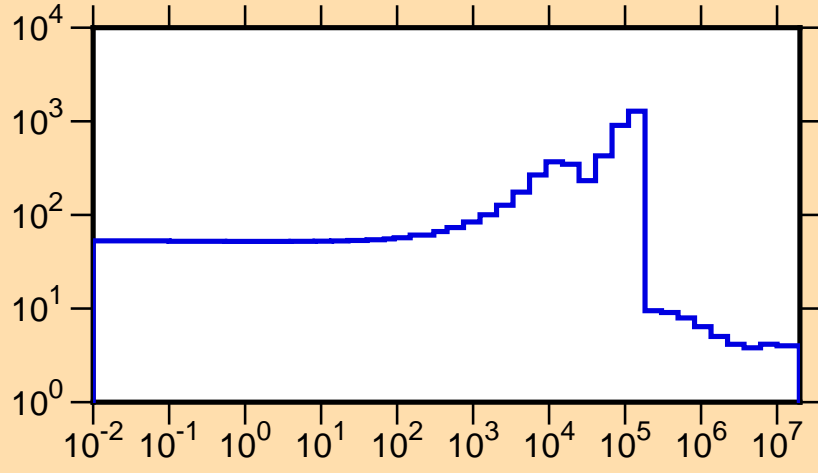
\sigma vs. E for ^{96}\text{Sr}(n,\text{tot.})
