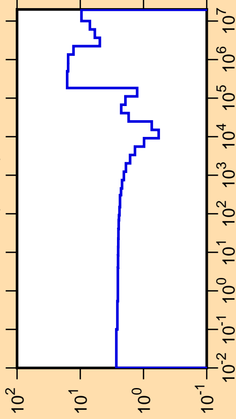
\Delta\sigma/\sigma vs. E for ^{96}\text{Sr}(n,\text{tot.})
