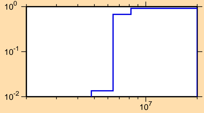
\sigma vs. E for ^{96}\text{Sr}(n,2n)
