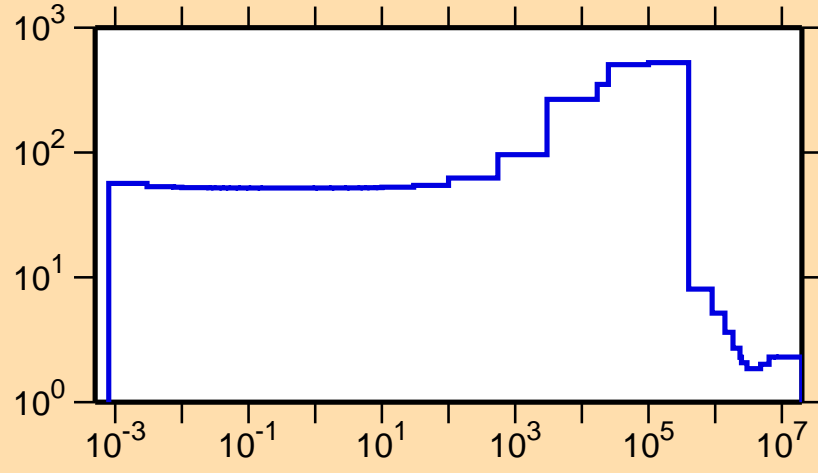
\sigma vs. E for ^{96}\text{Sr}(n,\text{el.})
