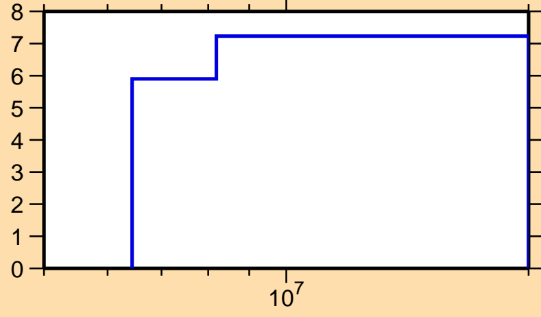
\Delta\sigma/\sigma vs. E for ^{96}\text{Sr}(n,\text{nonel.})
