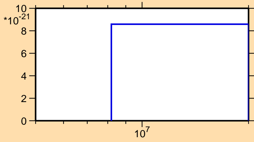
\sigma vs. E for ^{96}\text{Sr}(n,2np)
