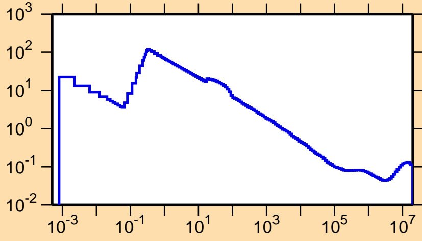
\sigma vs. E for ^{159}\text{Ta}(n,\alpha)
