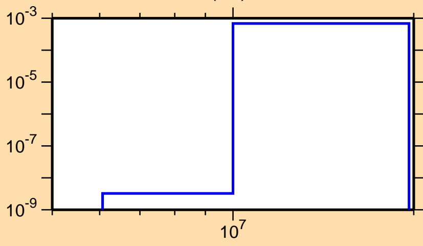
\sigma vs. E for ^{159}\text{Ta}(n,t)
