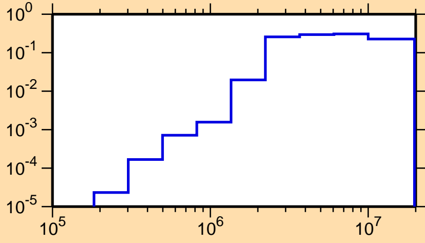
\sigma vs. E for ^{159}\text{Ta}(n,\text{inel.})
