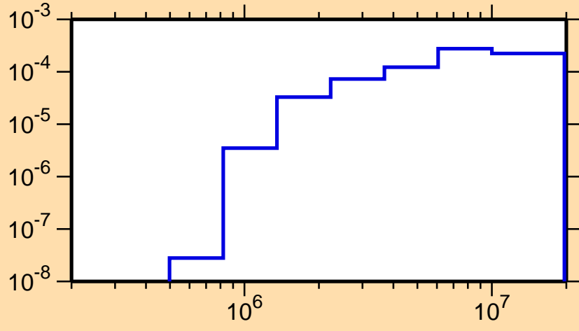
\sigma vs. E for ^{159}\text{Ta}(n,n_2)
