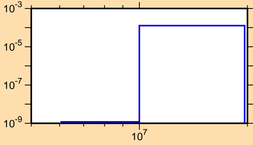
\sigma vs. E for ^{159}\text{Ta}(n,pd)
