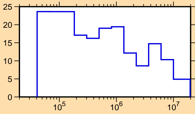
\Delta\sigma/\sigma vs. E for ^{159}\text{Ta}(n,\text{tot.})
