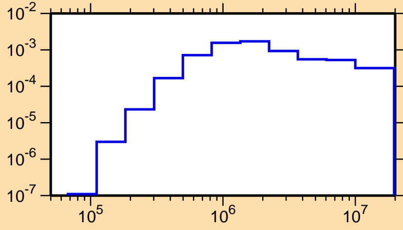
\sigma vs. E for ^{159}\text{Ta}(n,n_1)
