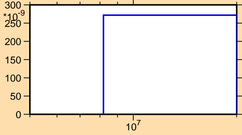
\sigma vs. E for ^{159}\text{Ta}(n,\text{nd})
