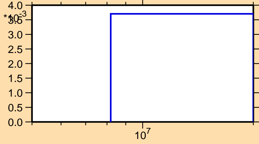
\sigma vs. E for ^{159}\text{Ta}(n,2n)
