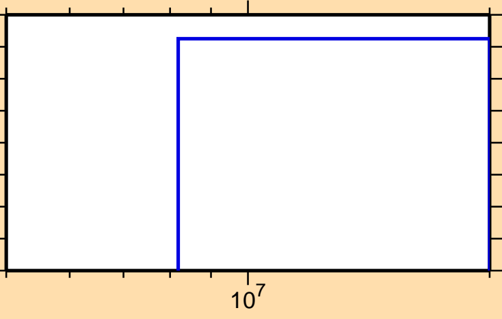
\sigma vs. E for ^{159}\text{Ta}(n,2np)
