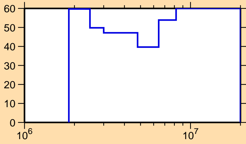
\Delta\sigma/\sigma vs. E for ^{159}\text{Ta}(n,n\text{cont.})
