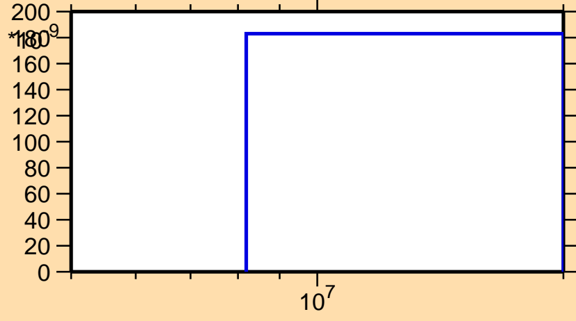
\sigma vs. E for ^{159}\text{Ta}(n,\text{pt})
