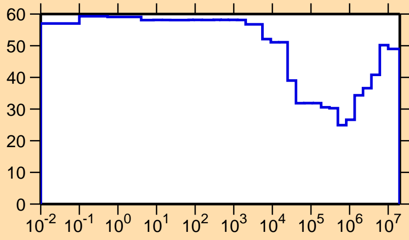
\Delta\sigma/\sigma vs. E for ^{160}\text{Ta}(n,p)
