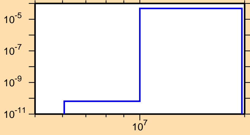
\sigma vs. E for ^{160}\text{Ta}(n,pd)
