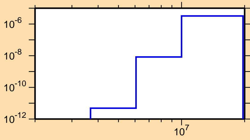
\sigma vs. E for ^{160}\text{Ta}(\text{mt117})
