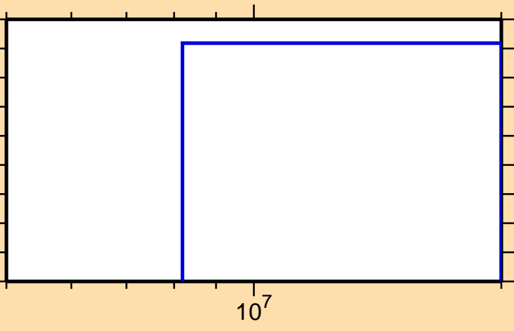
\sigma vs. E for ^{160}\text{Ta}(n,2np)
