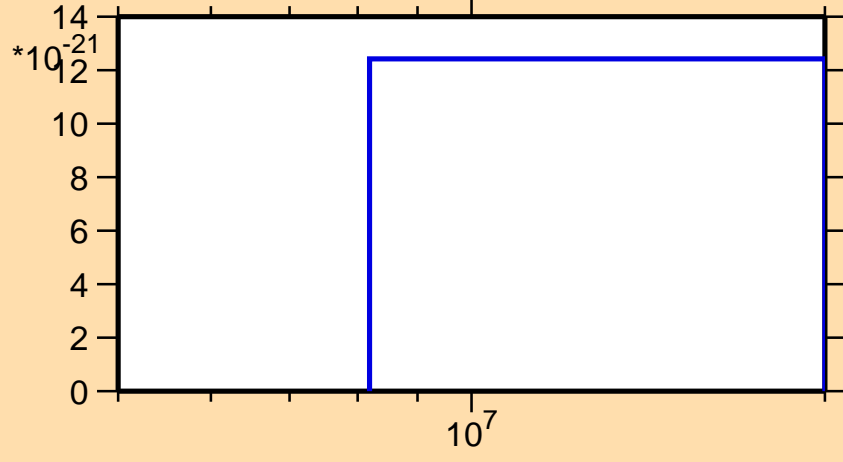
\sigma vs. E for ^{160}\text{Ta} (mt 11)
