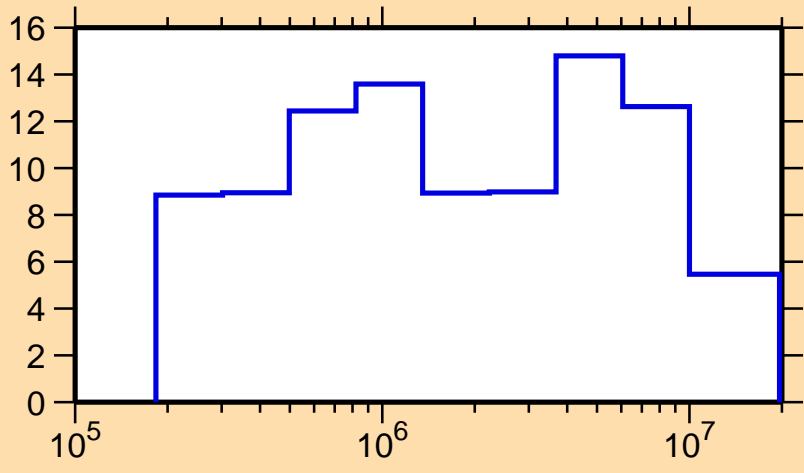
\Delta\sigma/\sigma vs. E for ^{160}\text{Ta}(n,tot.)
