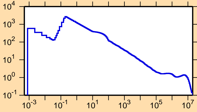
\sigma vs. E for ^{161}\text{Ta}(n,p)
