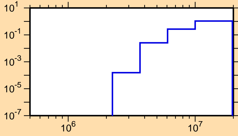
\sigma vs. E for ^{161}\text{Ta}(n,np)
