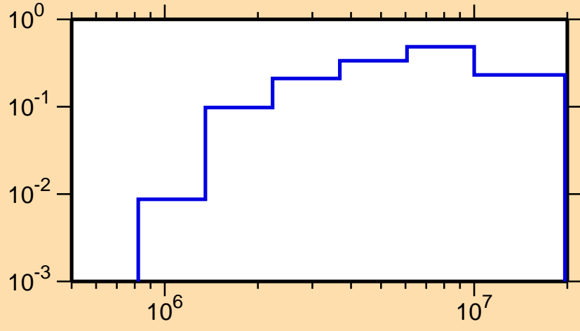
\sigma vs. E for ^{161}\text{Ta}(n,n\text{cont.})
