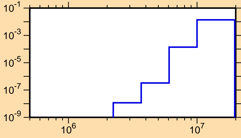
\sigma vs. E for ^{161}\text{Ta}(n,d)
