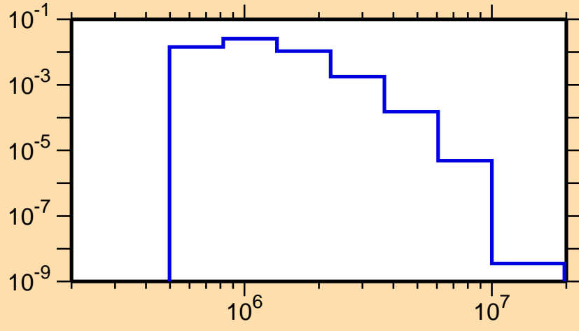
\sigma vs. E for ^{161}\text{Ta}(n,n_2)
