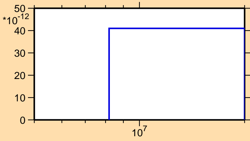
\sigma vs. E for ^{161}\text{Ta} (mt 34)
