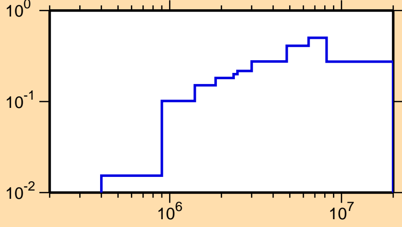
\sigma vs. E for ^{161}\text{Ta}(n,\text{inel.})
