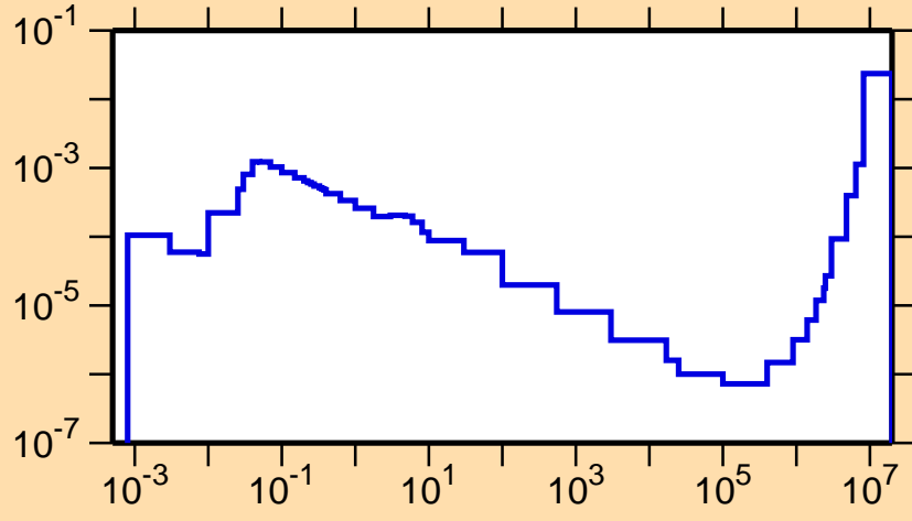
\sigma vs. E for ^{161}\text{Ta}(n,p\alpha)
