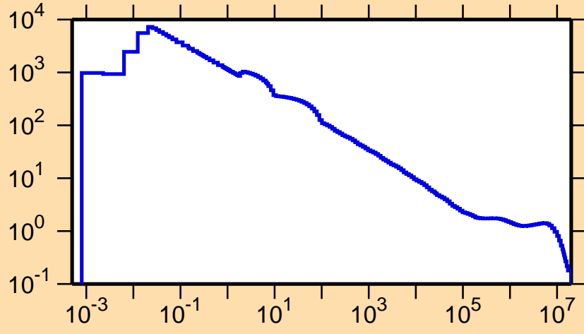
\sigma vs. E for ^{162}\text{Ta}(n,p)
