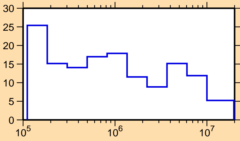
\Delta\sigma/\sigma vs. E for ^{162}\text{Ta}(n,\text{tot.})
