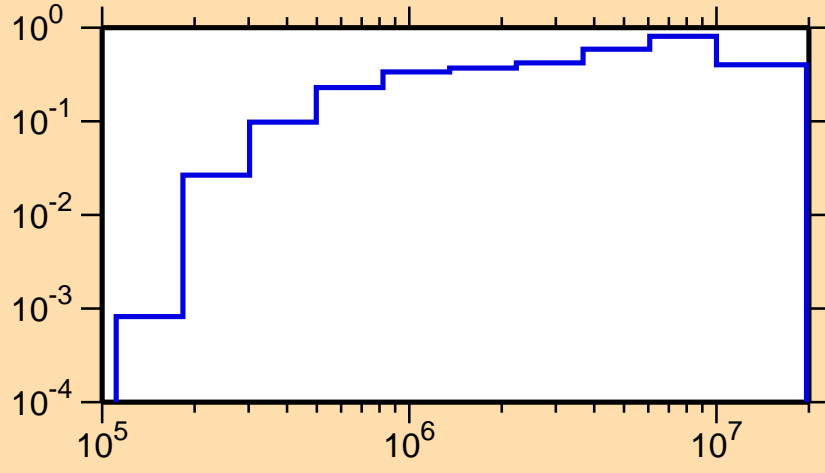
\sigma vs. E for ^{162}\text{Ta}(n,\text{inel.})
