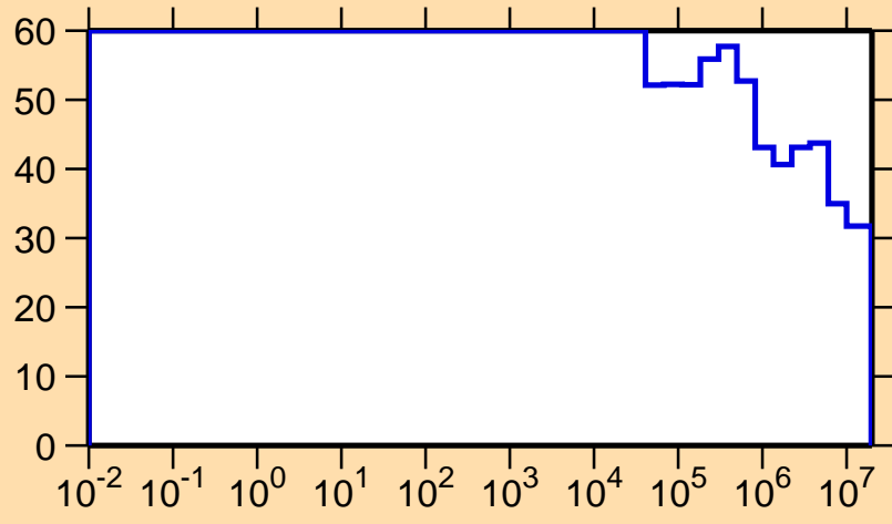
\Delta\sigma/\sigma vs. E for ^{162}\text{Ta}(n,p)
