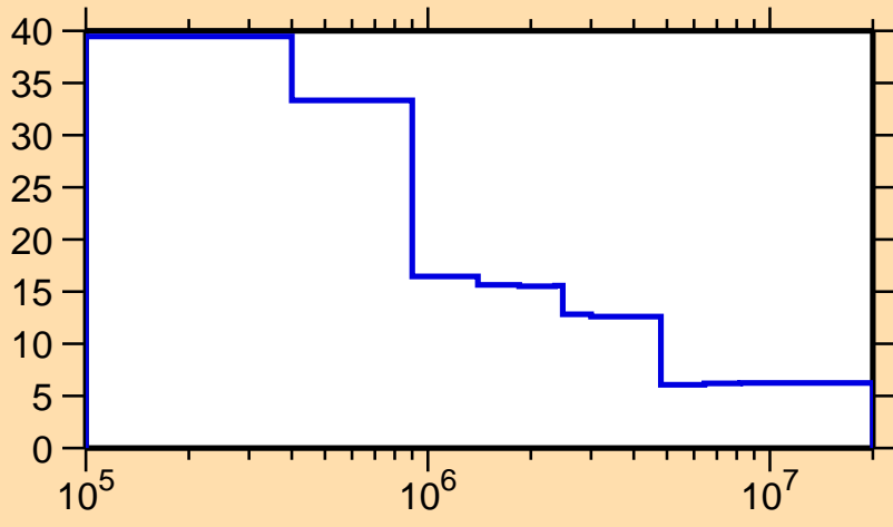
\Delta\sigma/\sigma vs. E for ^{162}\text{Ta}(n,\text{nonel.})
