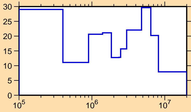
\Delta\sigma/\sigma vs. E for ^{162}\text{Ta}(n,\text{el.})
