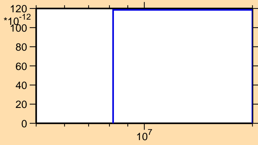
\sigma vs. E for ^{162}\text{Ta}(n,nt)
