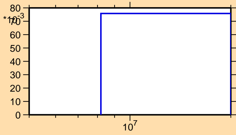
\sigma vs. E for ^{162}\text{Ta}(n,2n)
