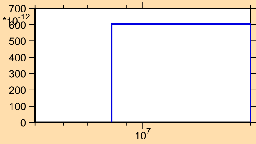
\sigma vs. E for ^{162}\text{Ta} (mt 34)
