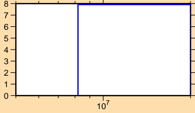
\Delta\sigma/\sigma vs. E for ^{162}\text{Ta}(n,\text{el.})
