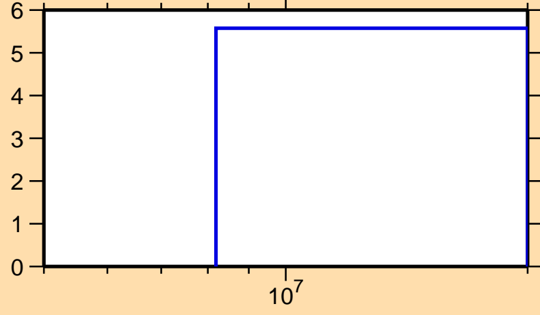
\Delta\sigma/\sigma vs. E for ^{162}\text{Ta}(n,\text{tot.})
