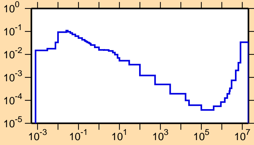
\sigma vs. E for ^{162}\text{Ta}(n,p\alpha)
