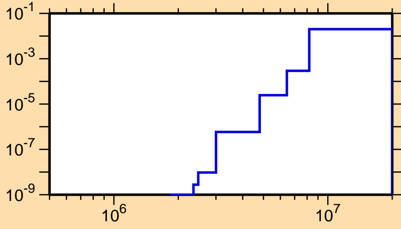
\sigma vs. E for ^{162}\text{Ta}(n,n\alpha)
