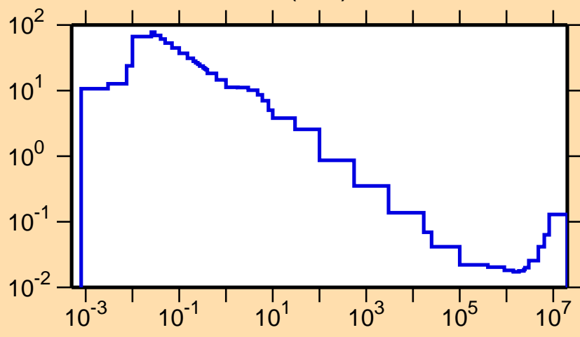
\sigma vs. E for ^{162}\text{Ta}(n,\alpha)
