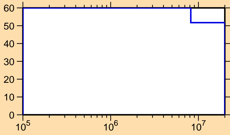
\Delta\sigma/\sigma vs. E for ^{162}\text{Ta}(n,n_1)
