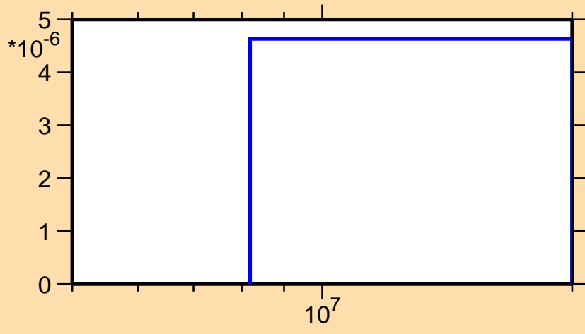
\sigma vs. E for ^{162}\text{Ta}(n,\text{nd})
