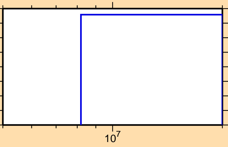
\sigma vs. E for ^{162}\text{Ta}(n,\text{pt})
