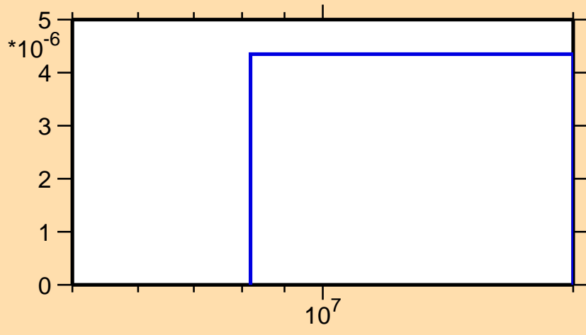
\sigma vs. E for ^{162}\text{Ta}(n,pd)
