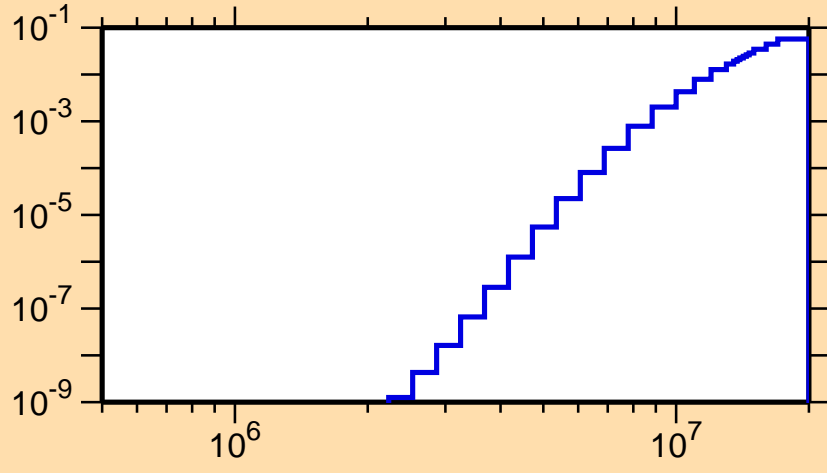
\sigma vs. E for ^{163}\text{Ta}(n,n\alpha)
