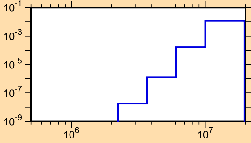
\sigma vs. E for ^{163}\text{Ta}(n,d)
