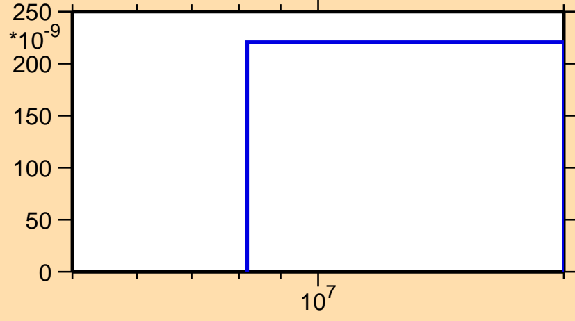
\sigma vs. E for ^{163}\text{Ta}(n,\text{nd})
