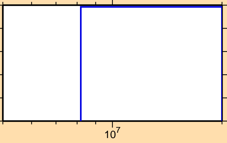
\sigma vs. E for ^{163}\text{Ta}(n,pd)
