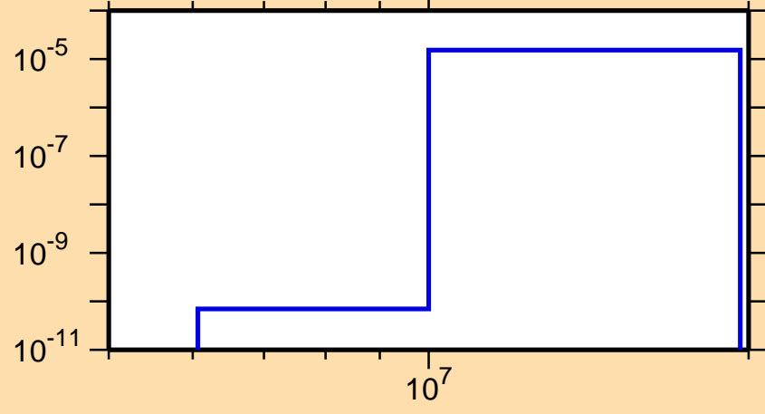
\sigma vs. E for ^{164}\text{Ta} (mt 45)
