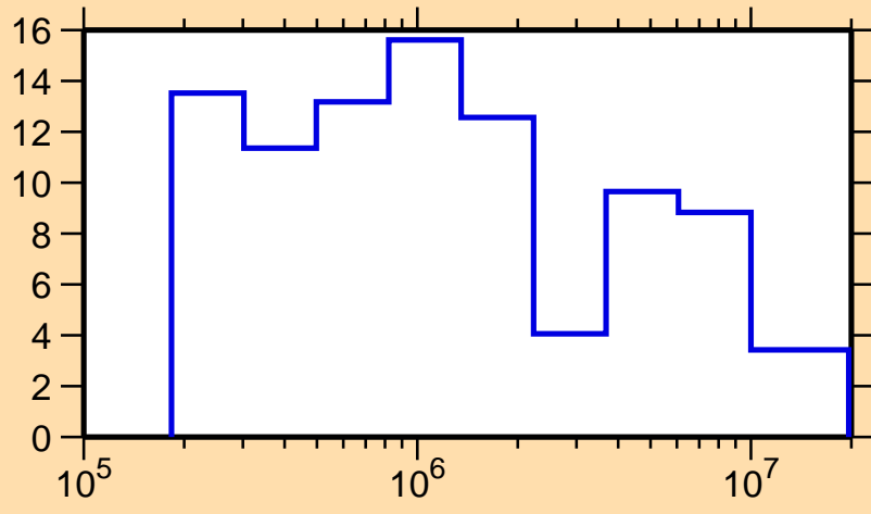
\Delta\sigma/\sigma vs. E for ^{164}\text{Ta}(n,tot.)
