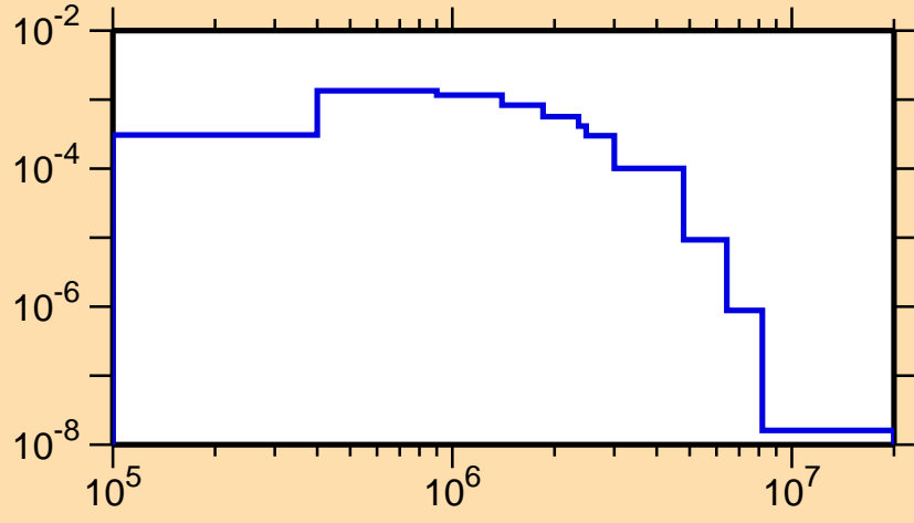
\sigma vs. E for ^{164}\text{Ta}(n,n_2)
