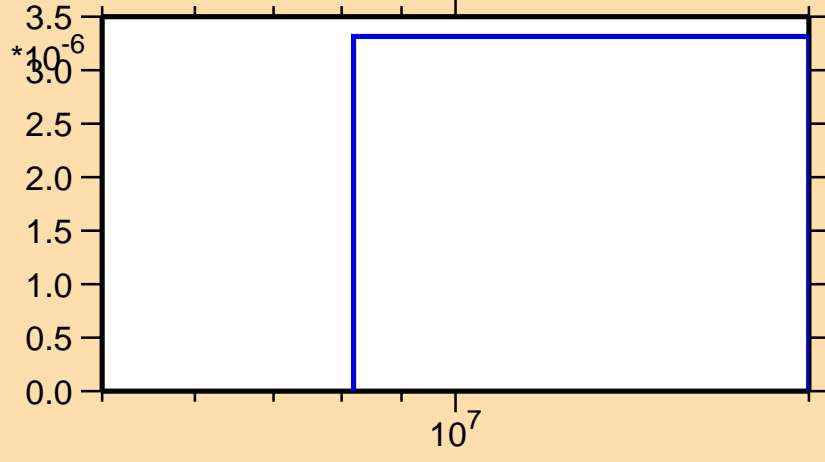
\sigma vs. E for ^{164}\text{Ta}(n,\text{nd})
