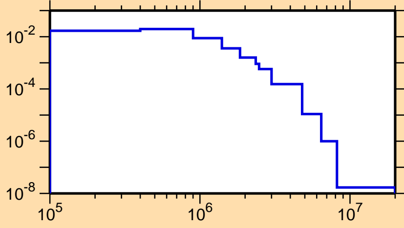
\sigma vs. E for ^{164}\text{Ta}(n,n_4)
