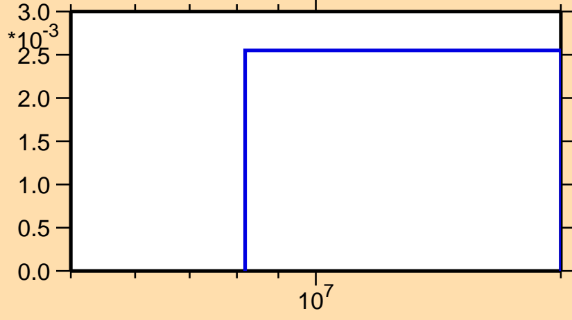
\sigma vs. E for ^{164}\text{Ta}(n,2np)
