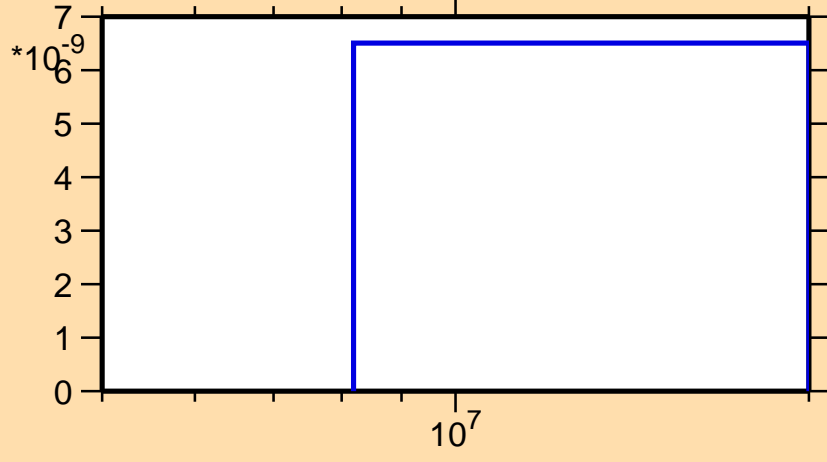
\sigma vs. E for ^{164}\text{Ta}(n,\text{pt})
