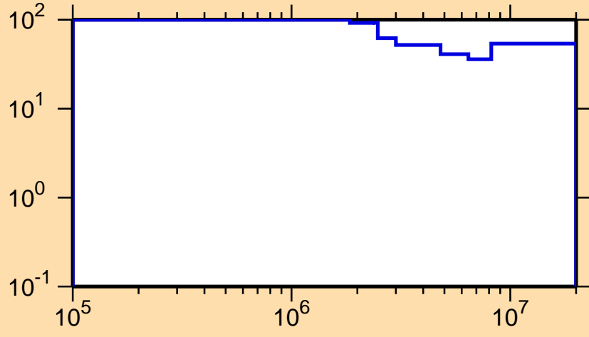
\Delta\sigma/\sigma vs. E for ^{164}\text{Ta}(n,n\text{cont.})
