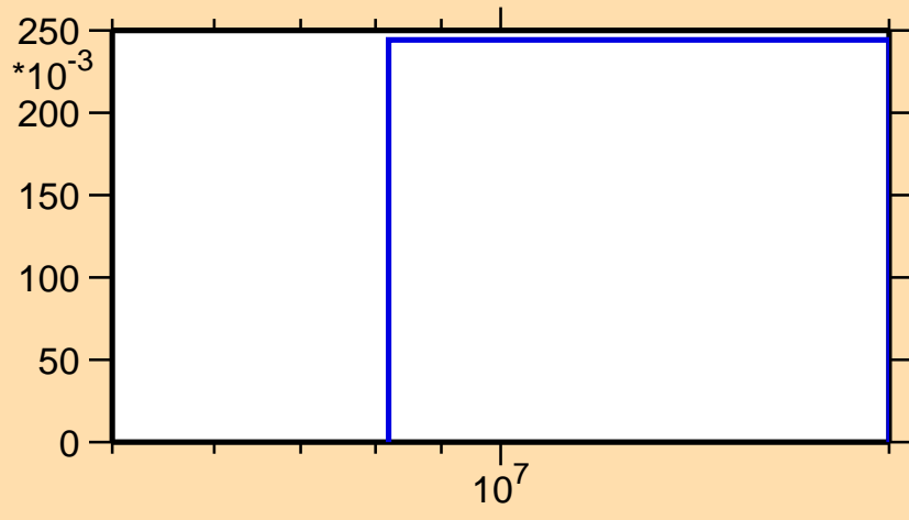
\sigma vs. E for ^{164}\text{Ta}(n,2n)
