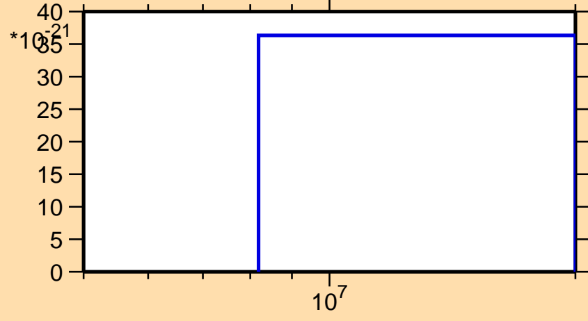
\sigma vs. E for ^{164}\text{Ta}(\text{mt } 11)
