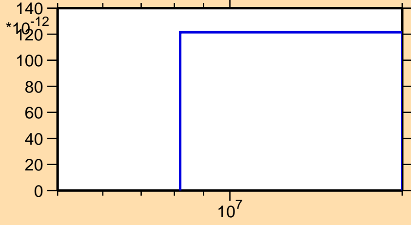
\sigma vs. E for ^{164}\text{Ta}(n,nt)
