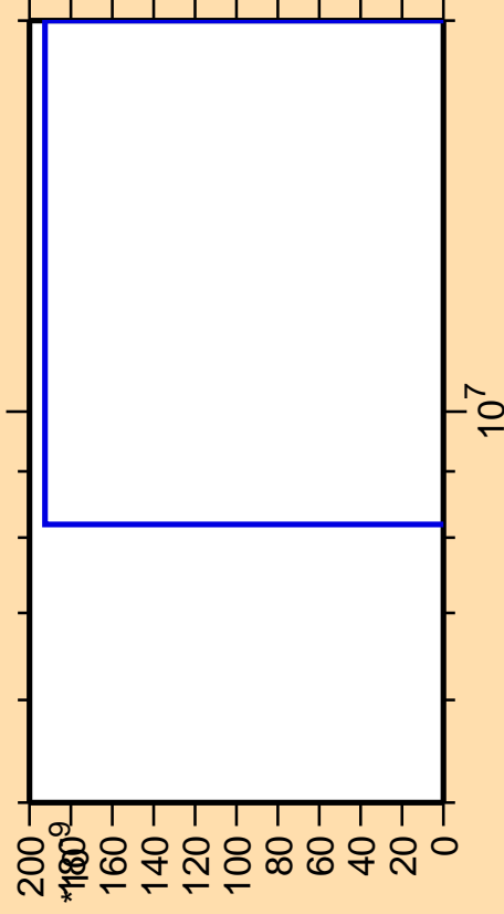
\Delta\sigma/\sigma vs. E for ^{164}\text{Ta}(\text{mt } 11)
