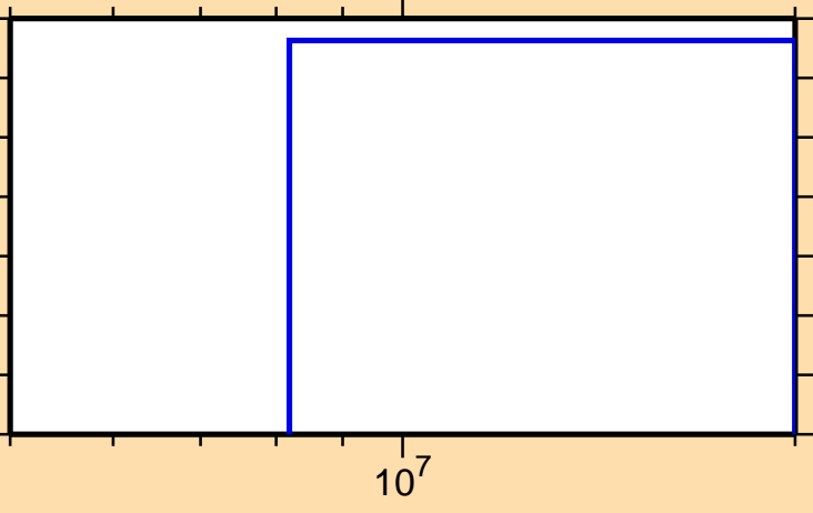
\sigma vs. E for ^{164}\text{Ta}(n,\text{nd})
