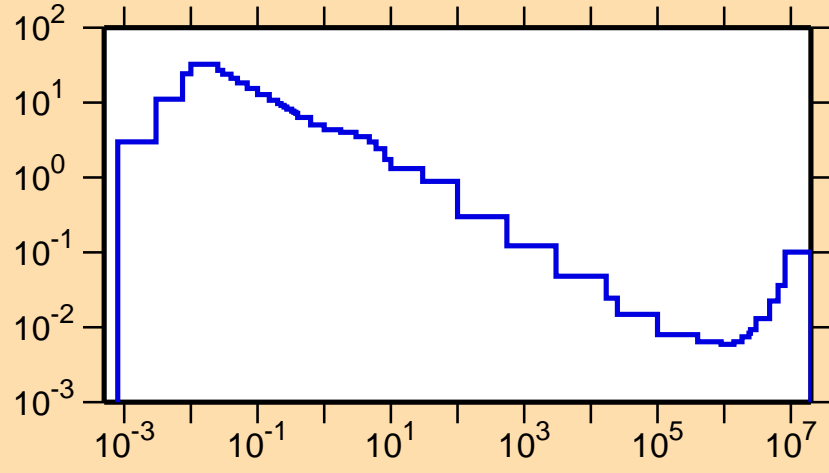
\sigma vs. E for ^{164}\text{Ta}(n,\alpha)
