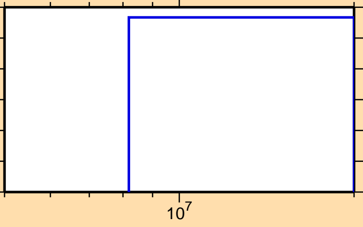
\sigma vs. E for ^{165}\text{Ta}(n,2np)
