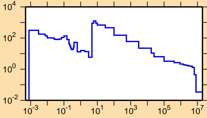
\sigma vs. E for ^{165}\text{Ta}(n,\gamma)
