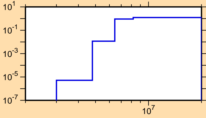
\sigma vs. E for ^{165}\text{Ta}(n,np)
