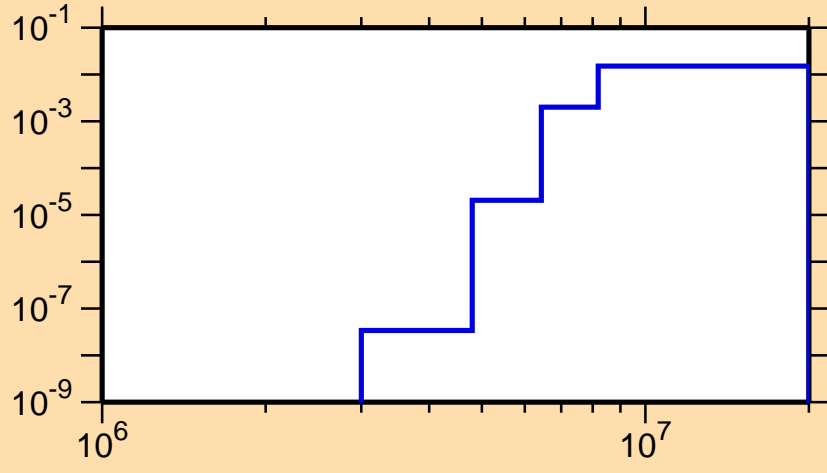
\sigma vs. E for ^{165}\text{Ta}(n,n\alpha)
