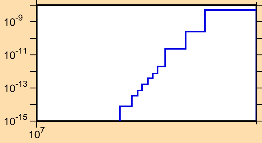
\sigma vs. E for ^{166}\text{Ta} (mt 34)
