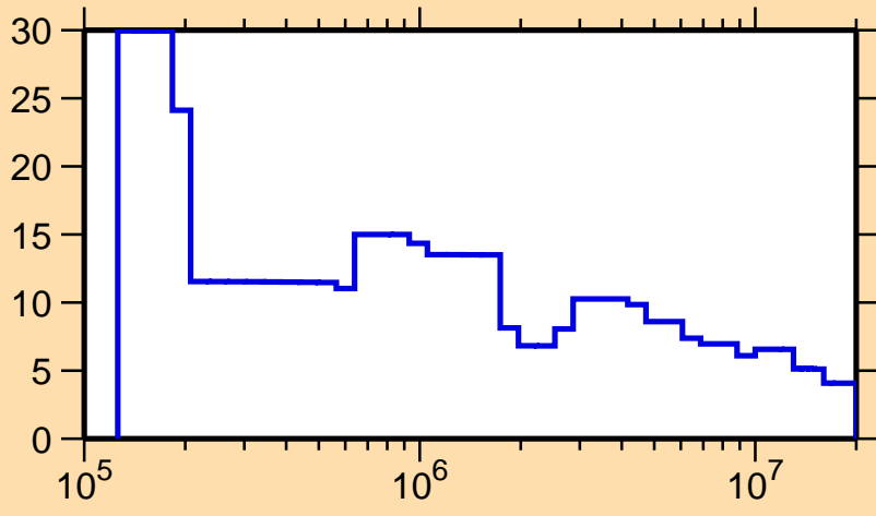
\Delta\sigma/\sigma vs. E for ^{166}\text{Ta}(n,\text{tot.})
