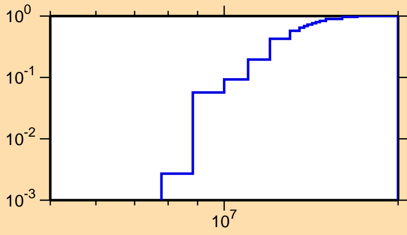
\sigma vs. E for ^{166}\text{Ta}(n,2n)
