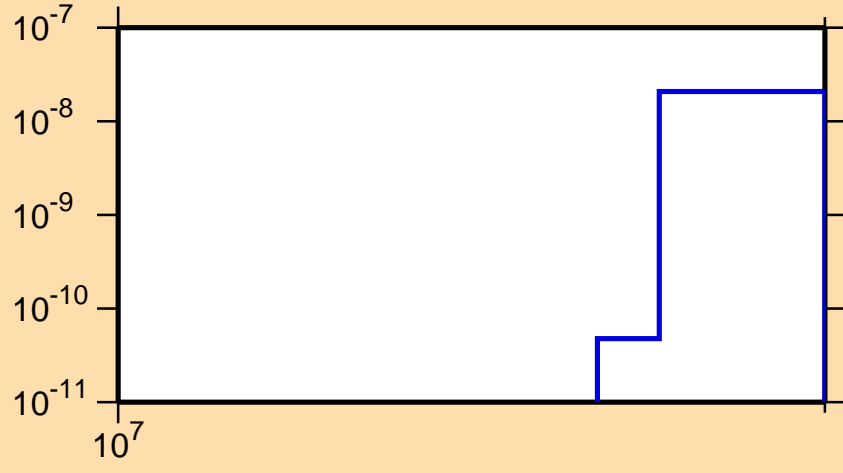
\sigma vs. E for ^{166}\text{Ta}(n,nt)
