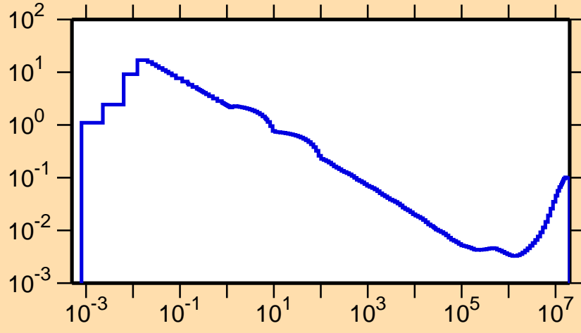
\sigma vs. E for ^{166}\text{Ta}(n,\alpha)
