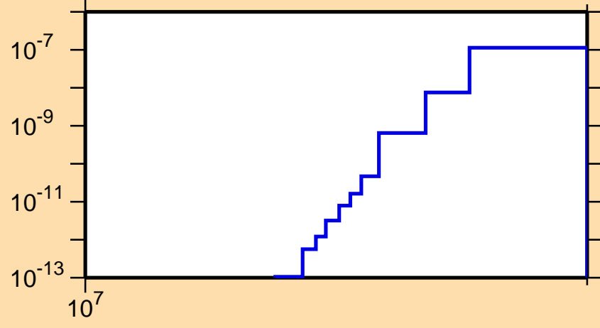
\sigma vs. E for ^{166}\text{Ta}(n,\text{pt})
