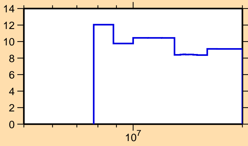
\Delta\sigma/\sigma vs. E for ^{166}\text{Ta}(n,\text{el.})
