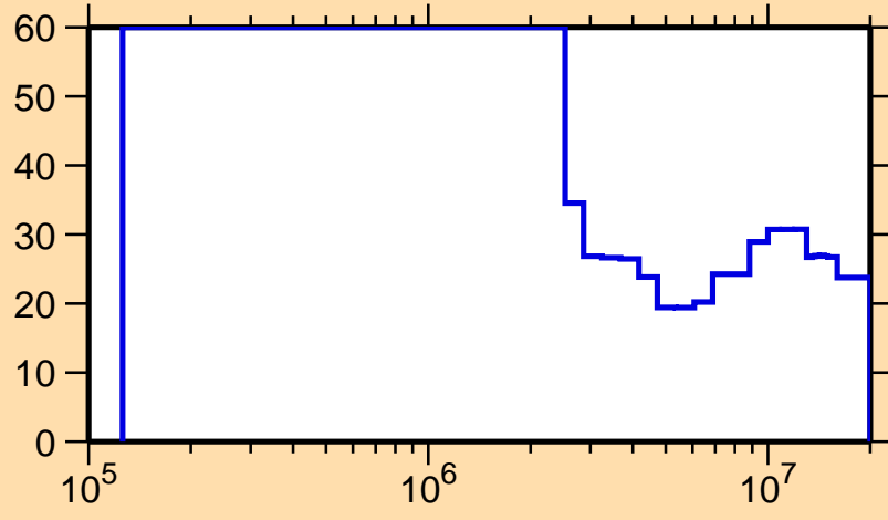
\Delta\sigma/\sigma vs. E for ^{166}\text{Ta}(n,\text{inel.})
