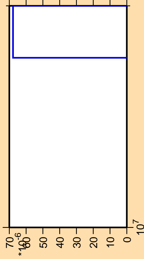
\Delta\sigma/\sigma vs. E for ^{166}\text{Ta} (mt 11)
