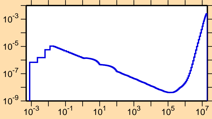
\sigma vs. E for ^{166}\text{Ta}(n,p\alpha)
