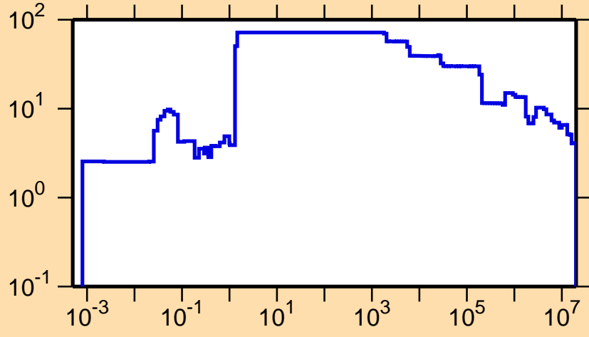
\Delta\sigma/\sigma vs. E for ^{166}\text{Ta}(n,\text{tot.})
