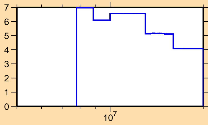
\Delta\sigma/\sigma vs. E for ^{166}\text{Ta}(n,\text{tot.})
