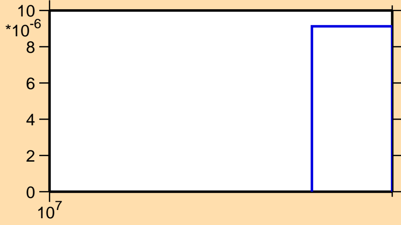
\sigma vs. E for ^{166}\text{Ta}(n,3n)
