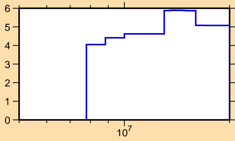
\Delta\sigma/\sigma vs. E for ^{166}\text{Ta}(n,\text{nonel.})
