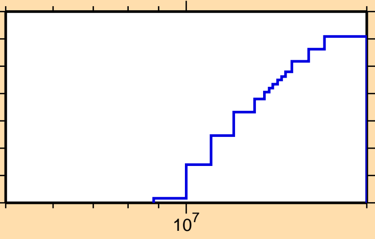
\sigma vs. E for ^{166}\text{Ta}(\text{mt117})
