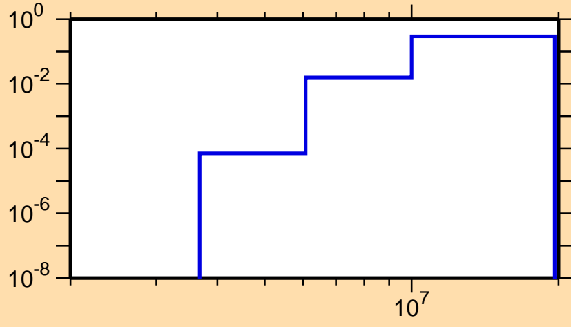
\sigma vs. E for ^{166}\text{Ta}(n,np)
