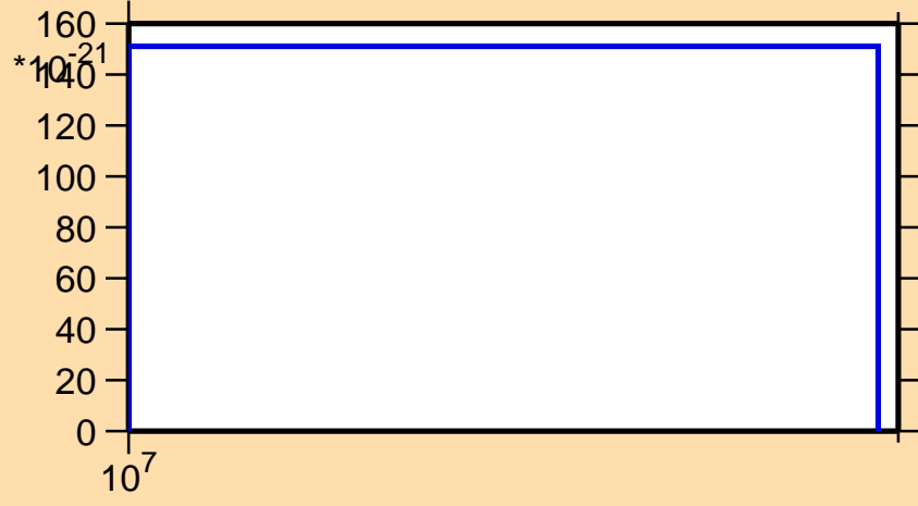
\sigma vs. E for ^{166}\text{Ta} (mt 11)
