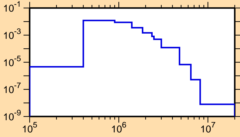
\sigma vs. E for ^{166}\text{Ta}(n,n_4)
