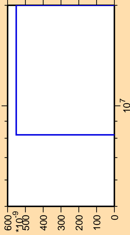
\Delta\sigma/\sigma vs. E for ^{166}\text{Ta}(\text{mt } 11)
