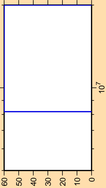
\Delta\sigma/\sigma vs. E for ^{166}\text{Ta}(n,3n)
