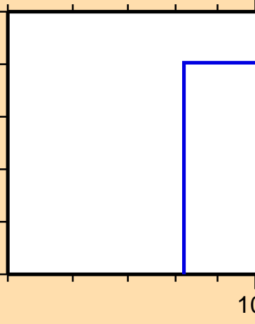
\sigma vs. E for ^{166}\text{Ta}(n,\text{nd})
