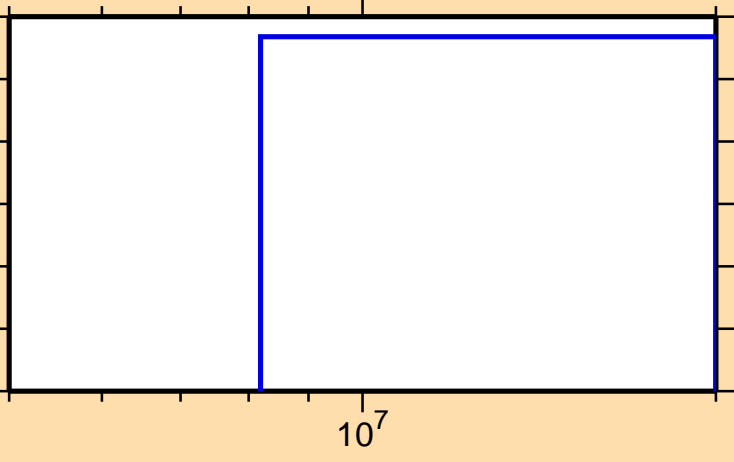
\sigma vs. E for ^{166}\text{Ta}(\text{mt117})
