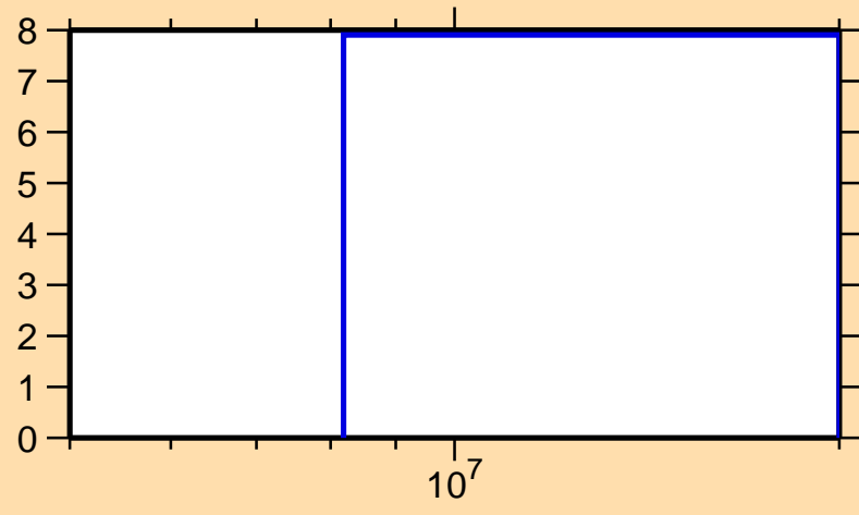
\Delta\sigma/\sigma vs. E for ^{166}\text{Ta}(n,\text{el.})
