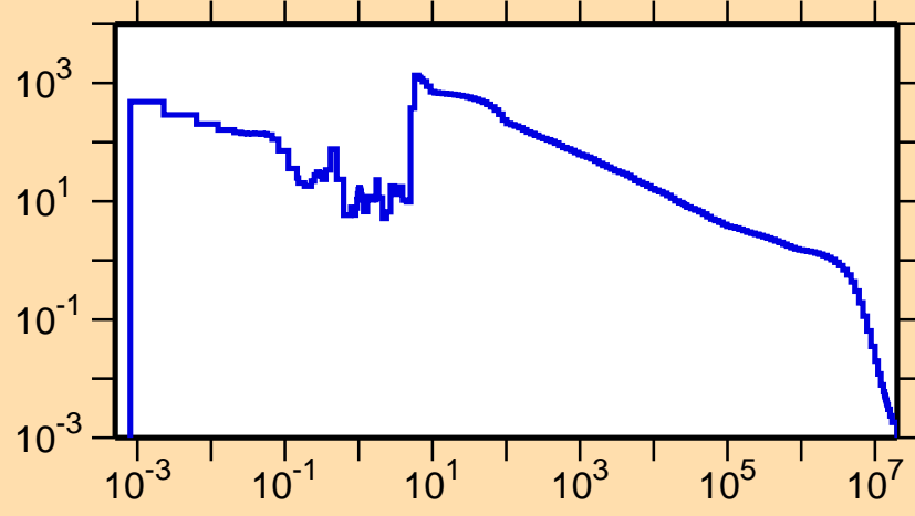
\sigma vs. E for ^{167}\text{Ta}(n,\gamma)
