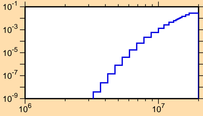
\sigma vs. E for ^{167}\text{Ta}(n,n\alpha)
