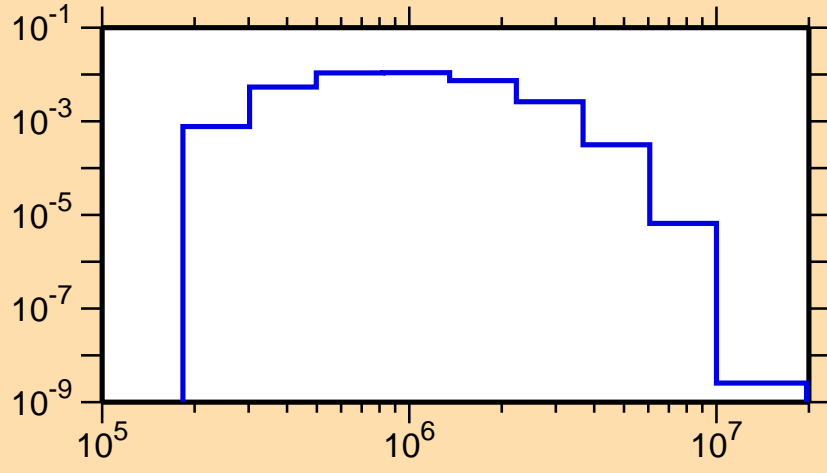
\sigma vs. E for ^{167}\text{Ta}(n,n_4)
