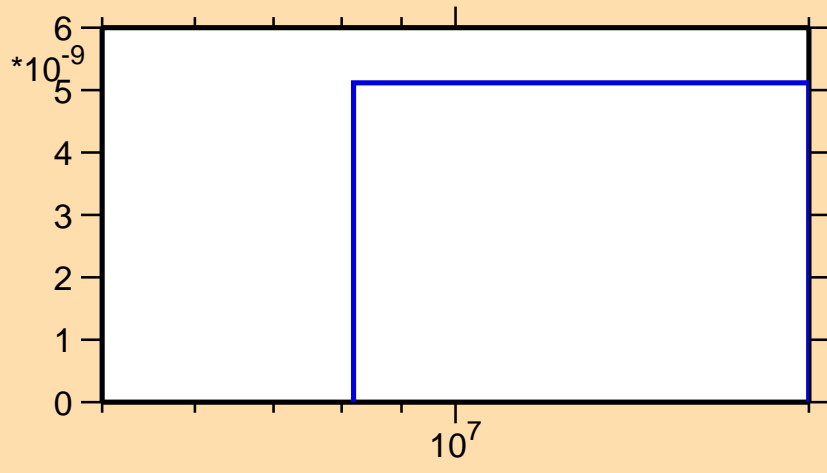
\sigma vs. E for ^{167}\text{Ta}(n,pd)
