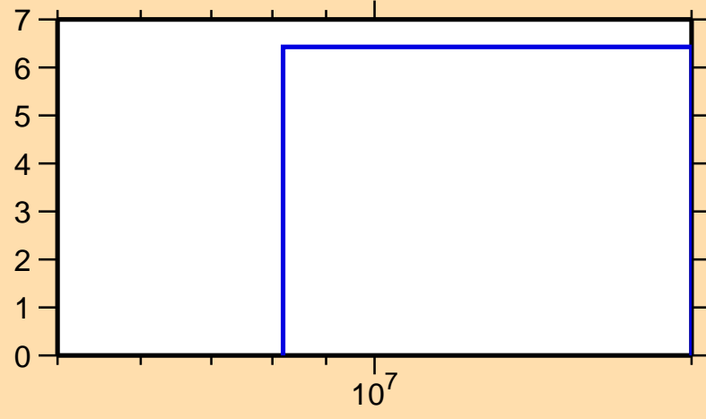
\Delta\sigma/\sigma vs. E for ^{167}\text{Ta}(n,\text{el.})
