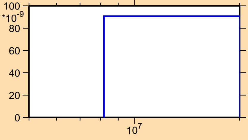
\sigma vs. E for ^{167}\text{Ta}(n,2n\alpha)
