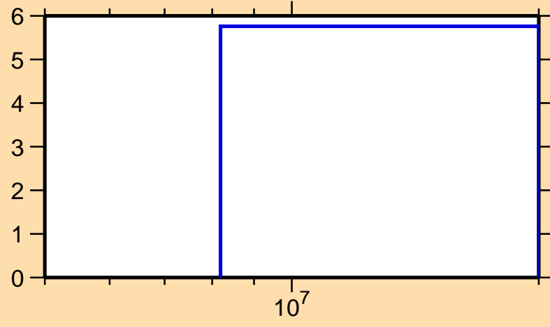
\Delta\sigma/\sigma vs. E for ^{167}\text{Ta}(n,\text{tot.})
